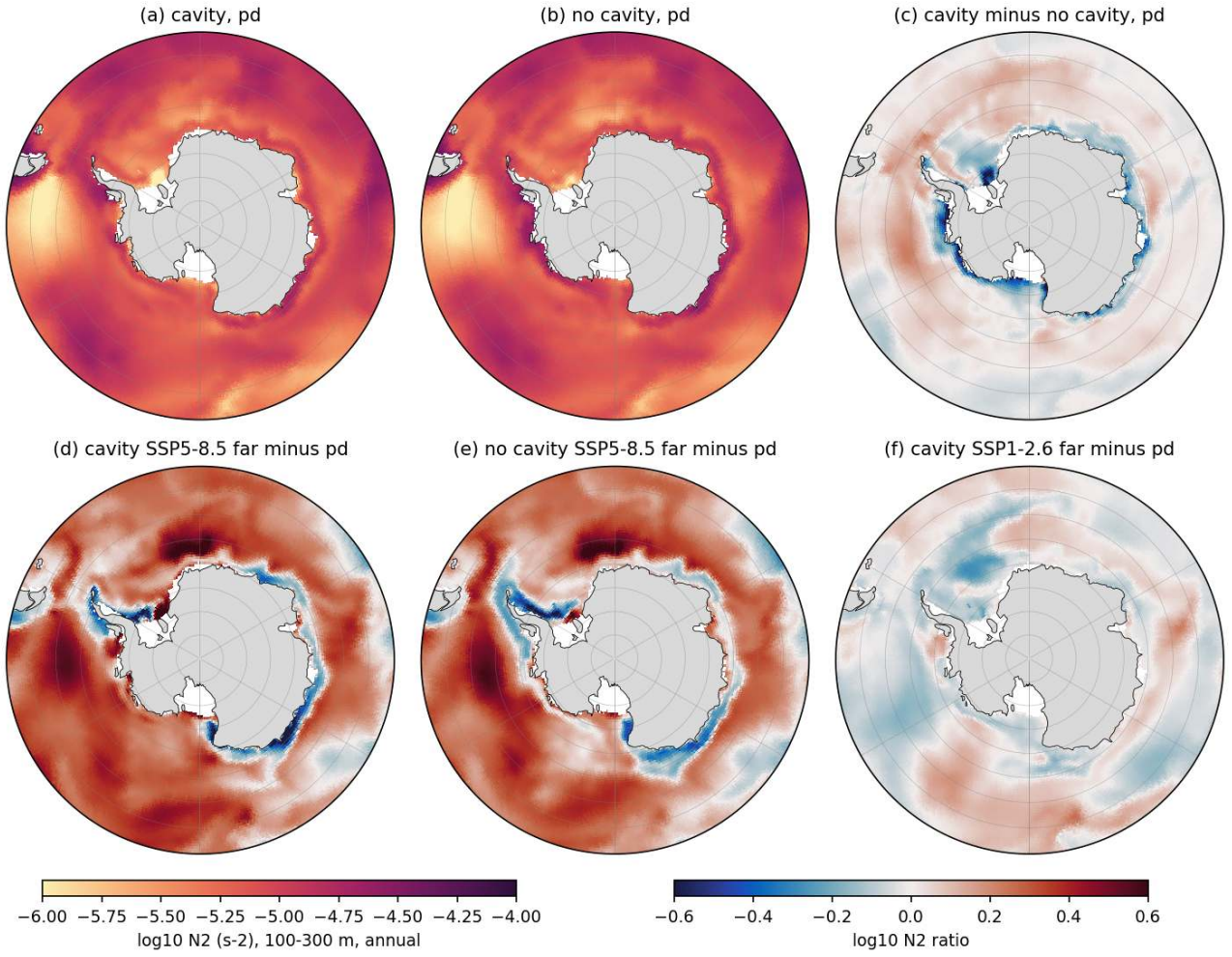
Figure 110: circ_N2_maps (circ). Maps south of 50S of log10 N2 averaged over 100-300 m (annual), same panel layout as above (cavity nodes excluded). Take-away: at pd the weakest 100-300 m stratification (N2 about 5\text{e-}6\text{ s-}2 ) is found over the Ross shelf in the cavity run ( 5.1\text{e-}6 versus 8.1\text{e-}6 in the no-cavity run) and near Maud Rise in the no-cavity run ( 4.7\text{e-}6 versus 5.3\text{e-}6 ), matching where each set convects. Under SSP5-8.5 N2 south of 60S increases by 60-70 percent (ssa mean 7.7\text{e-}6 to 1.28\text{e-}5 cavity, 7.9\text{e-}6 to 1.18\text{e-}5 no cavity), except on the East Antarctic and Ross shelves where it decreases (blue rings) as the winter halocline erodes.
