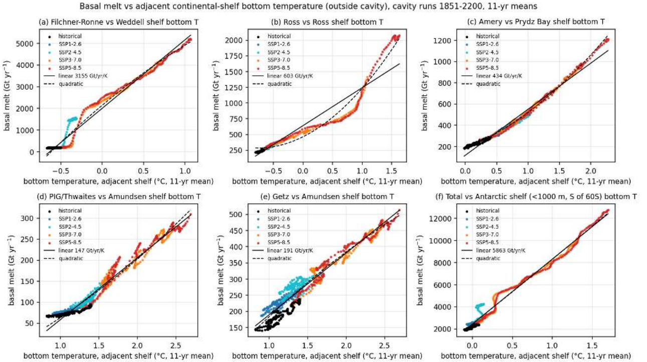
Figure 55: melt_vs_shelfT (melt). Scatter of 11-year mean basal melt against the 11-year mean bottom temperature of the adjacent continental-shelf region outside the cavity (cache bT, cavity nodes excluded) for all years 1851-2200 and all scenario chains (black historical, colours scenarios) with linear and quadratic fits. Filchner-Ronne vs Weddell shelf, Ross vs Ross shelf, Amery vs Prydz Bay shelf, PIG/Thwaites and Getz vs Amundsen shelf, total vs all Antarctic shelf (less than 1000 m, south of 60S). The Filchner-Ronne melt is a step function of Weddell shelf bottom temperature: below about -0.45 degC it stays near 200 Gt/yr, between -0.45 and -0.3 degC it jumps to 1500 to 2000 Gt/yr and above that it increases linearly at 3200 Gt/yr per K. Ross (600 Gt/yr per K, accelerating above 1 degC), Amery (430 Gt/yr per K), Getz (190) and PIG/Thwaites (150) respond quasi-linearly; the total responds at 5900 Gt/yr per K of Antarctic shelf bottom warming (250 percent per K relative to present day).
