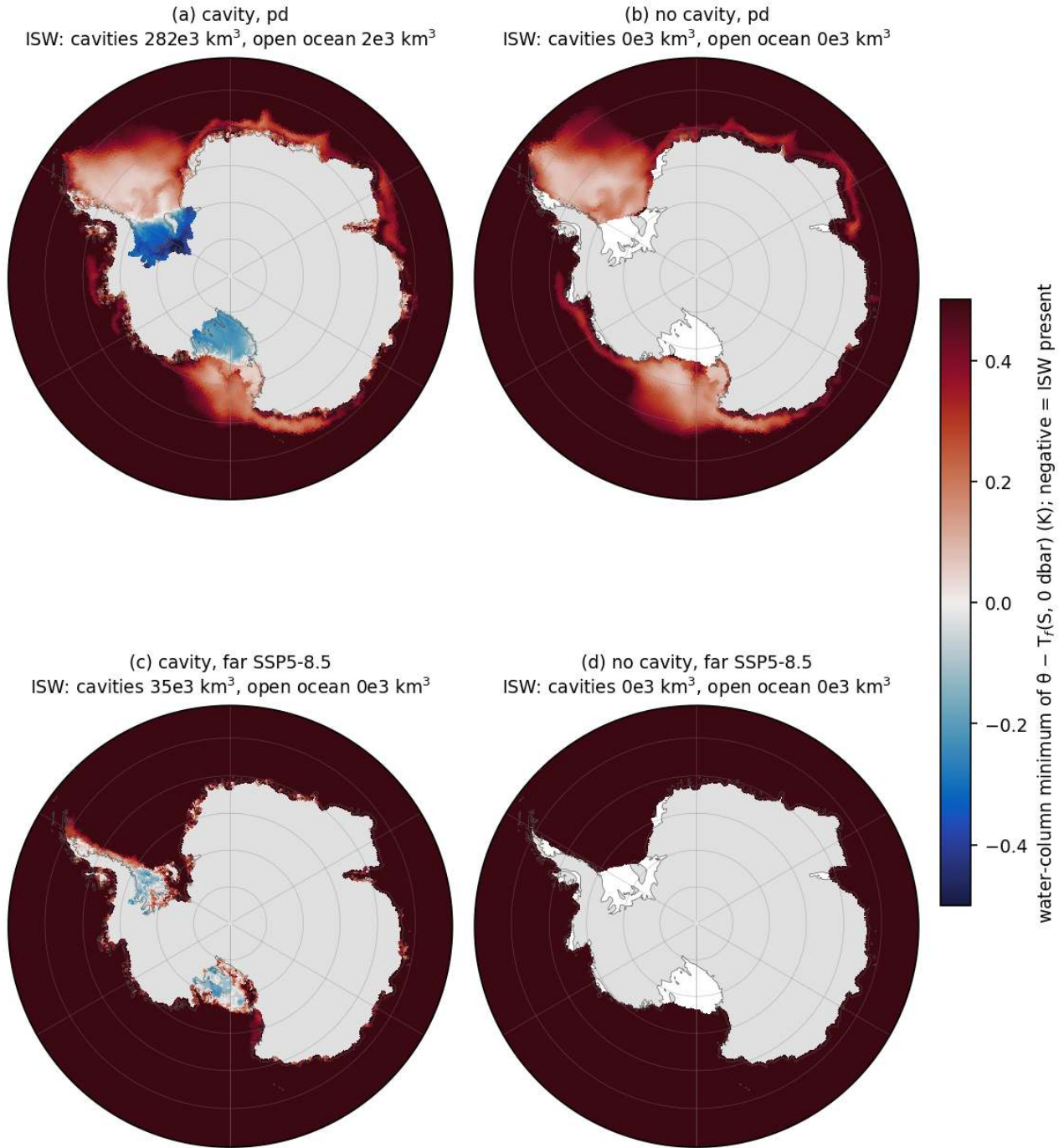
Figure 59: isw_maps (melt). Water-column minimum of theta minus the surface freezing point T_f(S, 0 \text{ dbar}) south of 60S (K, negative = Ice Shelf Water present) for the cavity run (a) pd and (c) far SSP5-8.5 and the no-cavity run (b) pd and (d) far SSP5-8.5 (30-year mean fields). ISW volumes inside the cavities and in the open ocean are given in the titles. ISW exists only inside the Filchner-Ronne, Ross and Amery cavities of the cavity run (282e3 km 3 at pd, 35e3 km 3 in far SSP5-8.5) and essentially nowhere in the open ocean in the 30-year mean fields; the no-cavity run has no water below the surface freezing point at all. Open-shelf water in front of the big cavities is within 0.1 to 0.2 K of the freezing point in the cavity run but 0.2 to 0.5 K above it in the no-cavity run.
