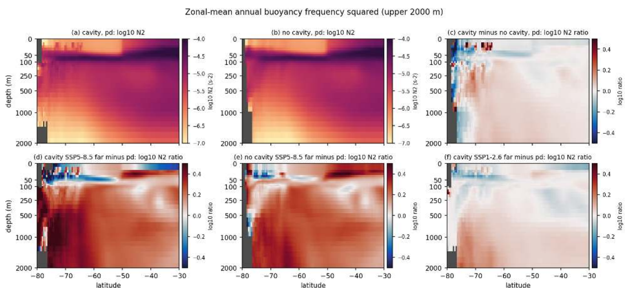
Figure 109: circ_N2_zonal (circ). Zonal-mean annual buoyancy frequency squared (log10 N2, interfaces) in the upper 2000 m. (a) cavity pd, (b) no cavity pd, (c) log10 ratio cavity/no cavity, (d, e) log10 ratio far SSP5-8.5 over pd, (f) far SSP1-2.6 over pd. Take-away: the pycnocline ( N2 > 1e-5 \text{ s}^{-2} ) sits at 50-150 m south of 60S and deepens to 500-1000 m north of 50S. The cavity run is slightly more stratified in the upper 300 m of the 70S-60S band (ratio 1.1-1.3); under SSP5-8.5 N2 in the upper 300 m south of 55S increases by a factor of 1.6-2.0 in both sets.
