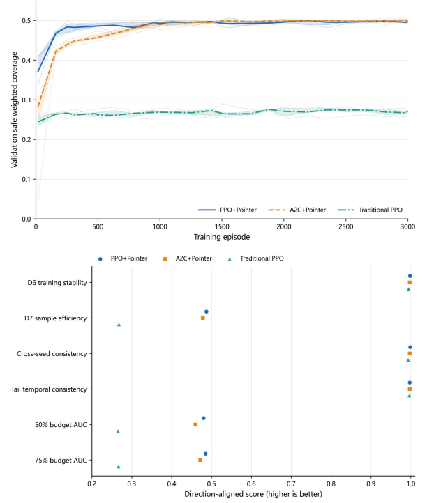
Figure 5. Corrected validation trajectories, training stability and sample efficiency. (a) Safe weighted coverage on the same fixed 108-task external validation set at 26 checkpoints over 3,000 episodes; thin curves are five seeds, heavy curves are medians and bands are interquartile ranges. (b) Corrected post-hoc D6 stability and D7 normalized validation-area-under-the-curve scores, together with direction-aligned component and budget-sensitivity values. These training dimensions supplement rather than redefine the confirmatory final-route endpoint.
