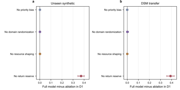
Figure 8. Four component ablations. Points are full-model minus ablation mean differences in map-level safe weighted coverage; horizontal intervals are 95% map-bootstrap intervals. Asterisk significance, where reported in the Source Data, follows Holm adjustment within the prespecified ablation family.
