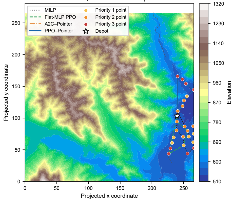
Fixed DSM task: terrain, road network and representative routes
