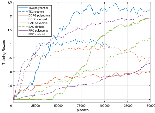
Fig. 11. Comparison of different training setups.
