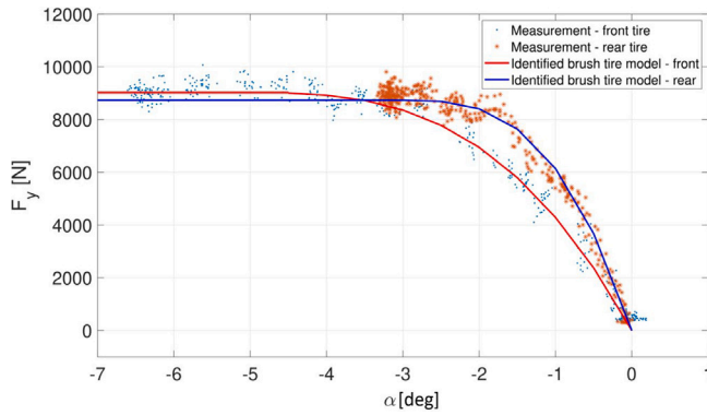
Fig. 9. Front and rear tire characteristics.
