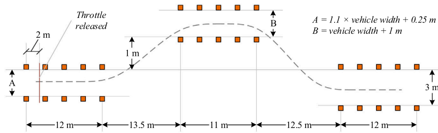
Fig. 1. The double lane-change maneuver according to ISO-3888-2 (International Organization for Standardization (ISO 3888-2:2011), 2011).
