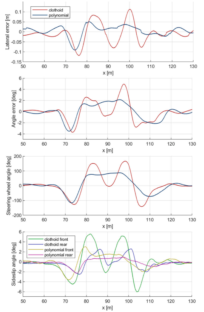
Fig. 16. MPC controller errors, steering wheel and sideslip angles of same initial speed of successful ISO 3888-2 experiments in simulation.
