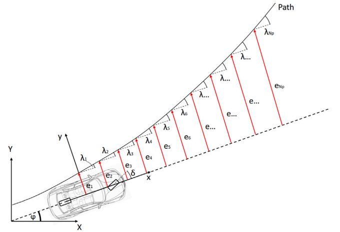
Fig. 10. Reference lateral error and orientation error in the ego frame.
