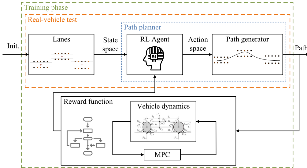
Fig. 2. Training architecture.
