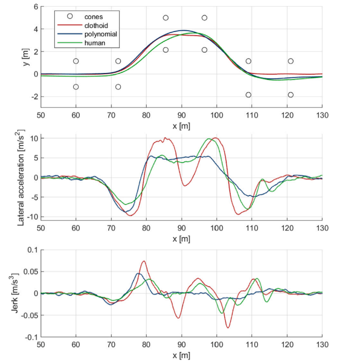
Fig. 14. Traversed routes and lateral accelerations of same initial speed of successful ISO 3888-2 experiments on the test track.
