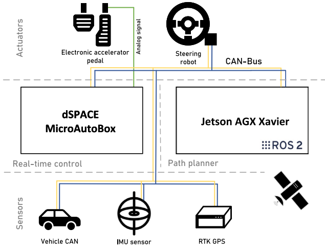
Fig. 7. System architecture of the experimental setup.
