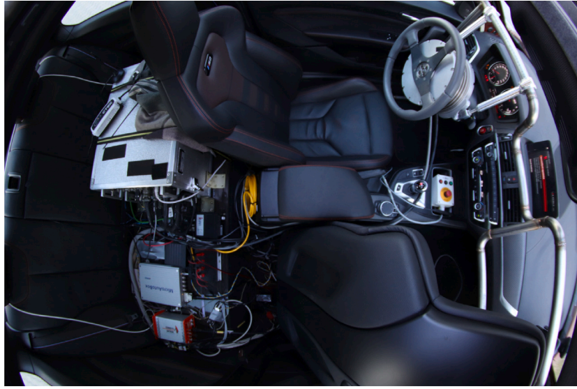
Fig. 8. Instrumentation and steering robot installation in the test vehicle.
