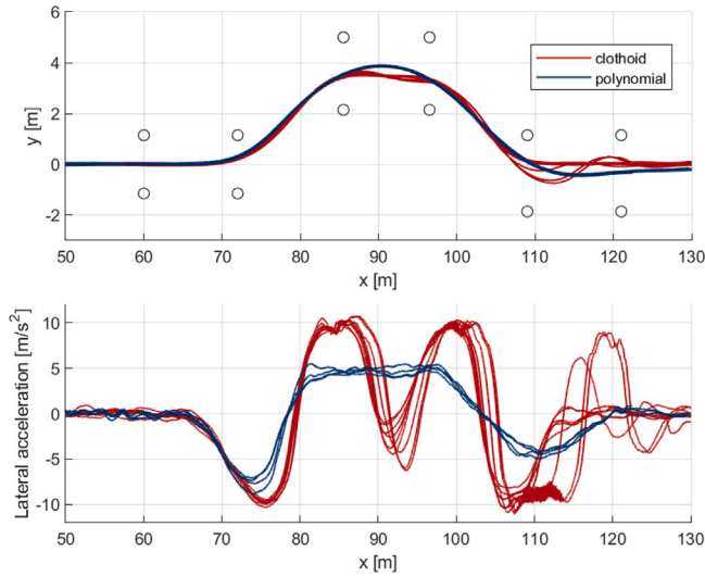
Fig. 15. Path and lateral acceleration comparison of the clothoid and polynomial based methods on the test track.
