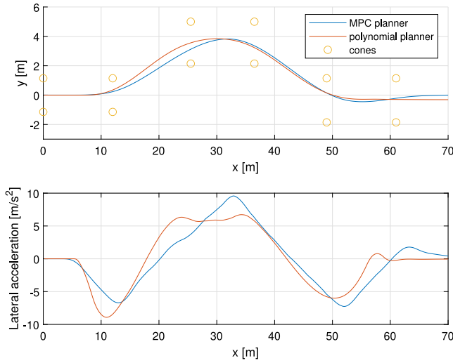
Fig. 12. Comparison of the performance of the polynomial and the pure Adaptive MPC planners in simulation.
