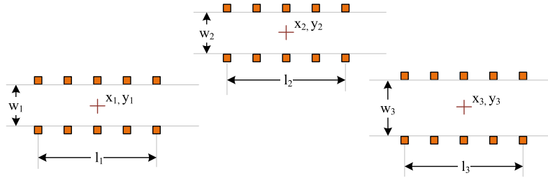
Fig. 4. State representation of the training environment.
