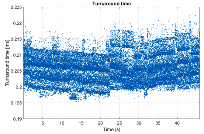
Fig. 13. MicroAutoBox turnaround time measurement of the path following MPC.
