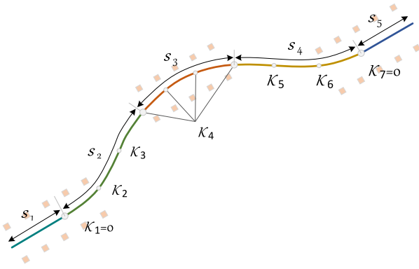
Fig. 6. The path built of polynomial and straight sections.
