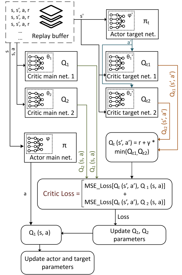
Fig. 3. TD3 training process.
