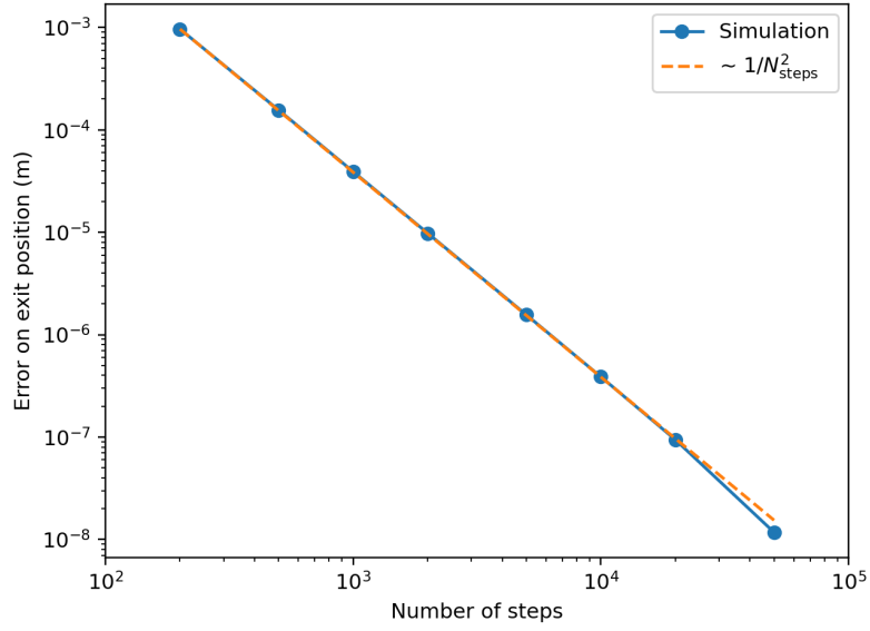
Figure 11.2: Convergence of the exit-position error for the linear-fringe solenoid. The dashed line shows a 1/N_{\text{steps}}^2 reference scaling.
