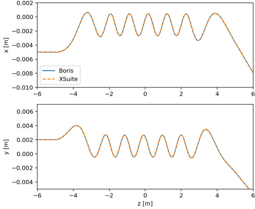
Figure 11.1: Comparison of the transverse position obtained with the spatial Boris integrator and with the Xsuite solenoid map.
