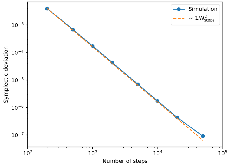
Figure 11.3: Convergence of the boundary symplectic deviation \|M^T S M - S\|_2 for the linear-fringe solenoid. The dashed line shows a 1/N_{\text{steps}}^2 reference scaling.
