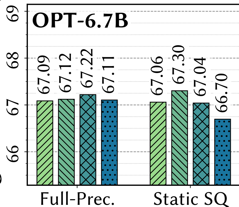
Avg. Zero-shot Acc. (%)
