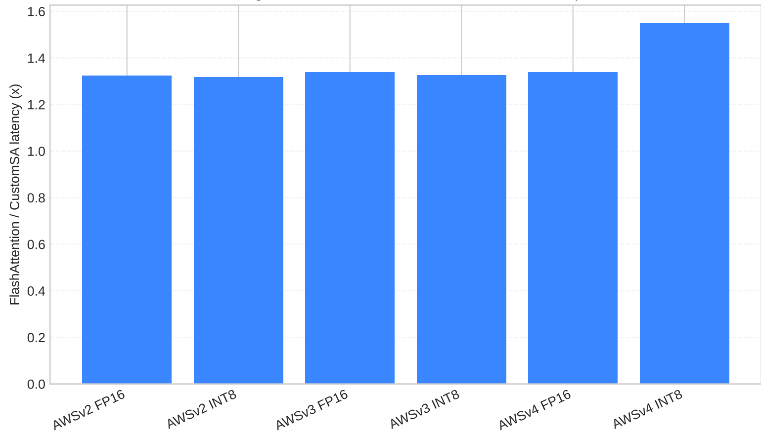
Longest-Context FlashAttention vs CustomSA Gap
