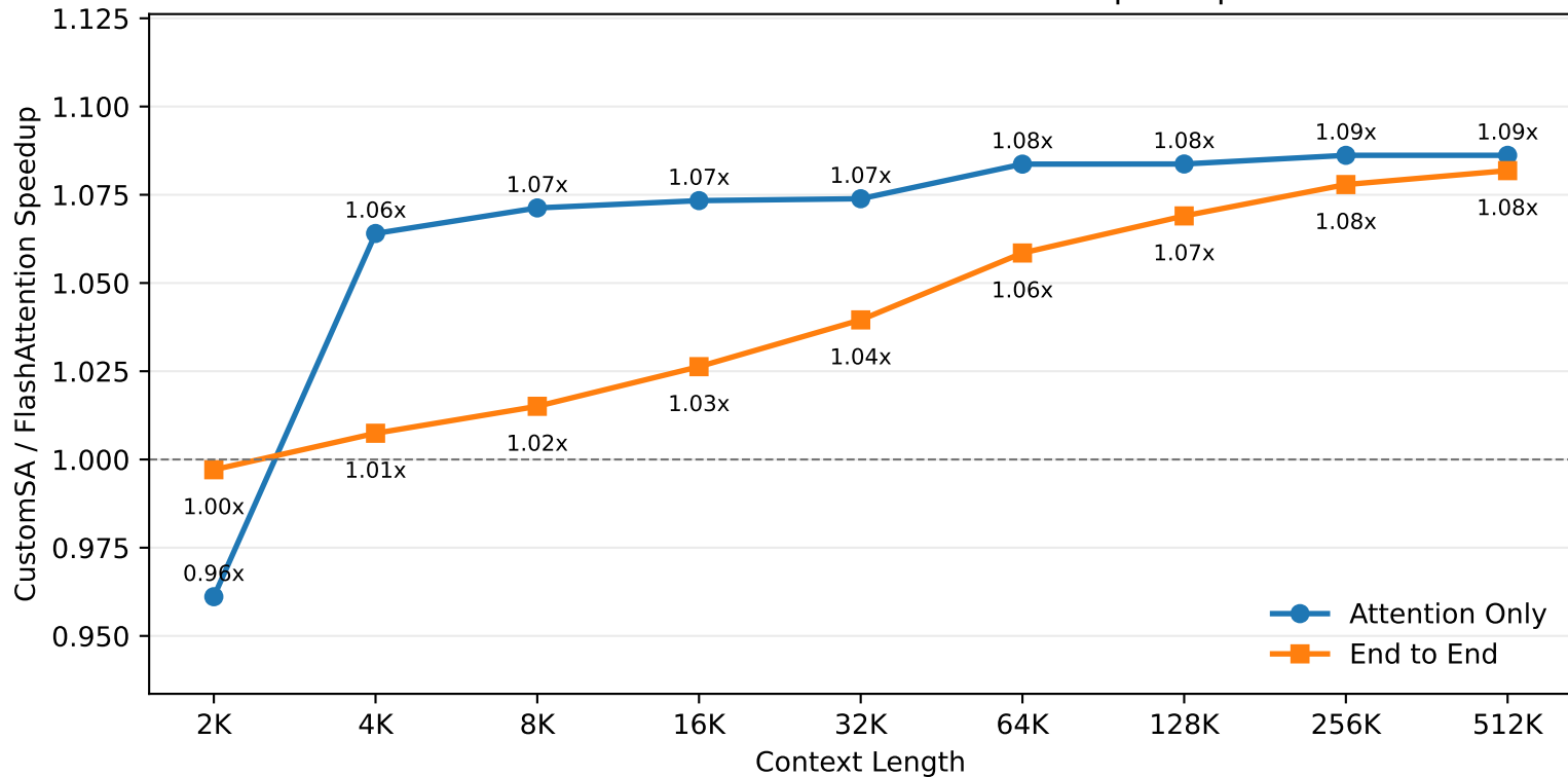
B300 CustomSA over FlashAttention Speedup
