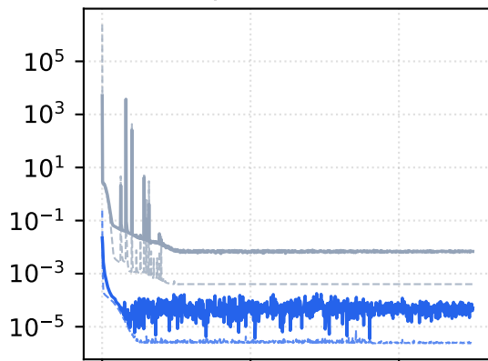
Rsqrt — 2264.3x
