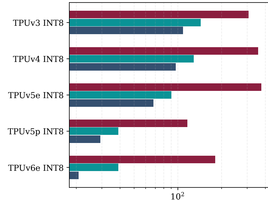
TPU INT8 @ 32k (No Conversion)
