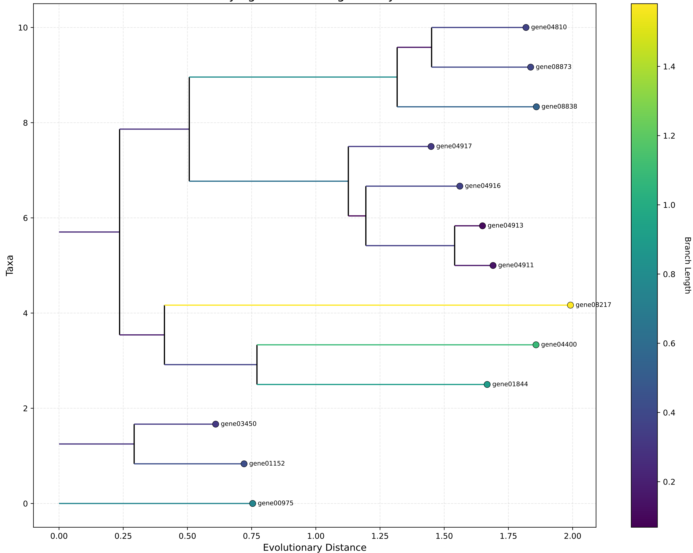
Phylogram - Rectangular Layout
