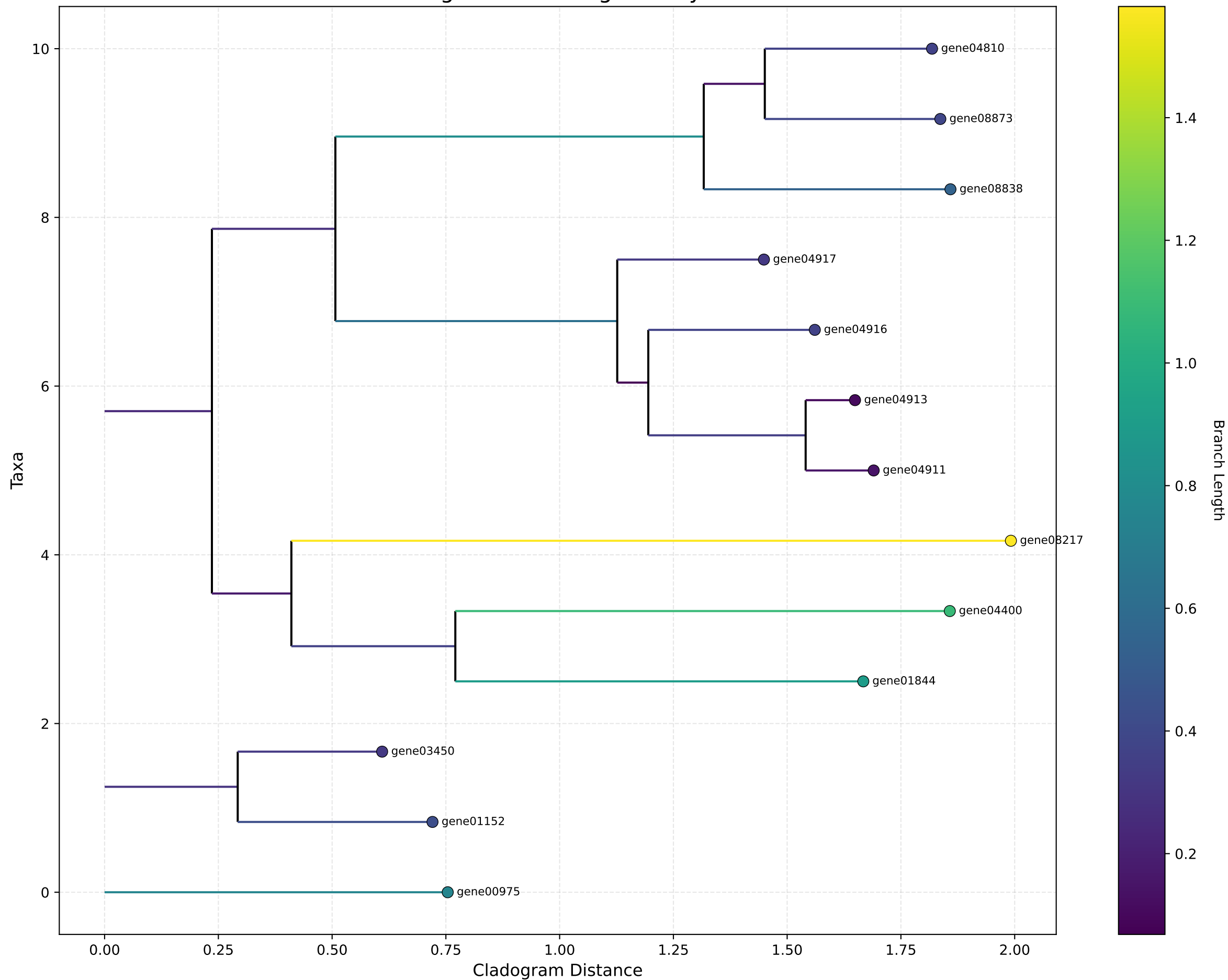
Cladogram - Rectangular Layout
