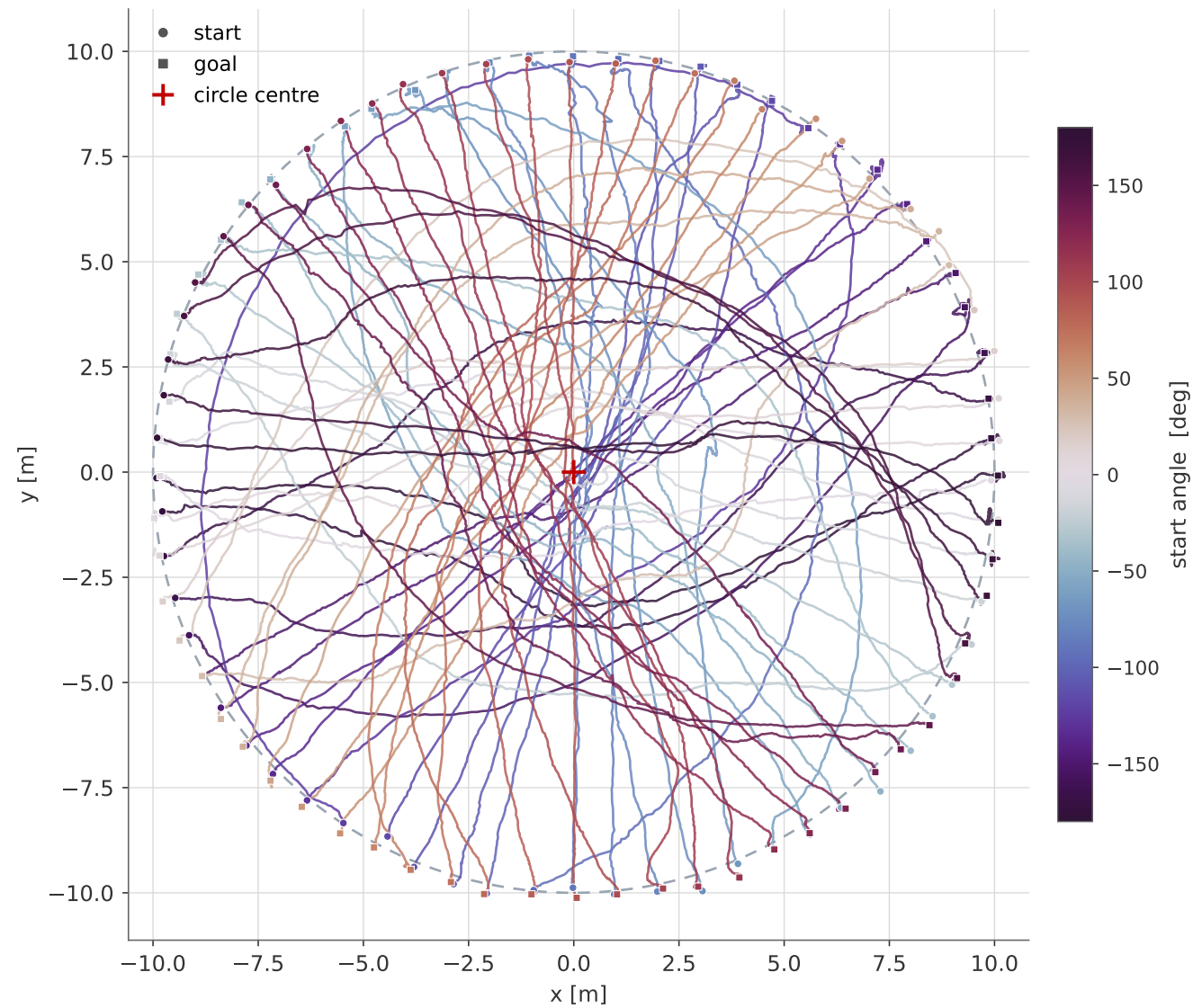
Circle antipodal — raw trajectories 64 pedestrians on a 10 m circle
