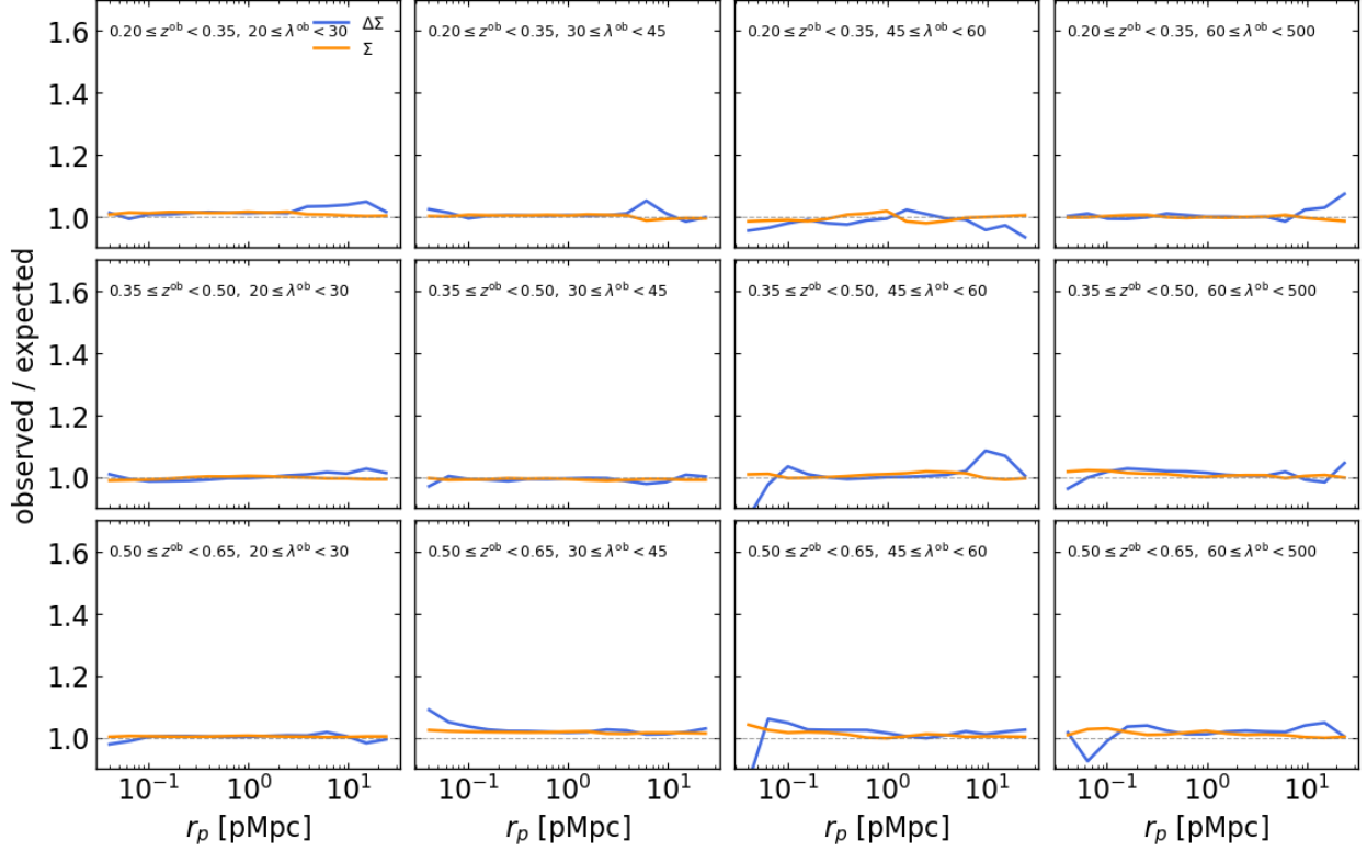
Figure 6: Null test: same Wu+22 panel grid but binning on the C19 sampler ( \lambda^{\text{ob}}, z^{\text{ob}} ) rather than the catalog ( \lambda^{\text{RM}}, z^{\text{RM}} ). The bell collapses to \approx 1 across all bins, confirming the R \sim 1 pMpc peak in Fig. 5 is genuinely LSS-driven.
