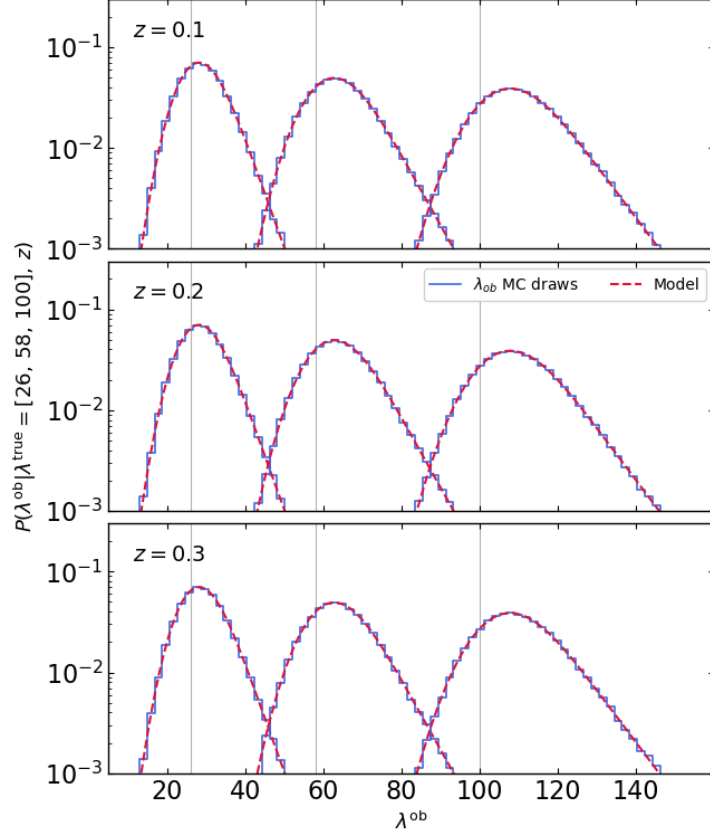
Figure 1: MC draws of \lambda^{\text{ob}} from sample_lambda_obs (blue histograms) overlaid with the closed-form C19 Eq. 6 PDF (red dashed) at three reference redshifts and three intrinsic richnesses. The two agree within Poisson noise across the bulk and the tail.
