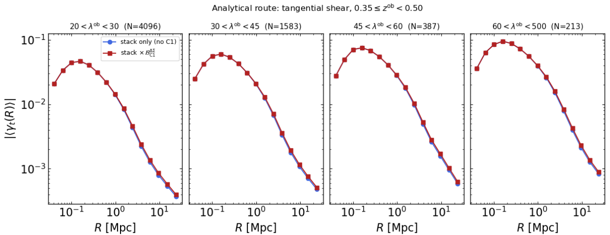
Figure 4: Analytical route: tangential shear in the middle redshift slice z^{\text{ob}} \in [0.35, 0.50) for each richness bin. Blue circles: \gamma_t from the unweighted C19-binned \Delta\Sigma stack (no correction). Red squares: same stack multiplied by \mathcal{B}_{\text{sel},\text{C1}}^{\Delta\Sigma}(R) . The C1 correction lifts the data vector by \sim 5\text{--}15\% depending on bin and scale.
