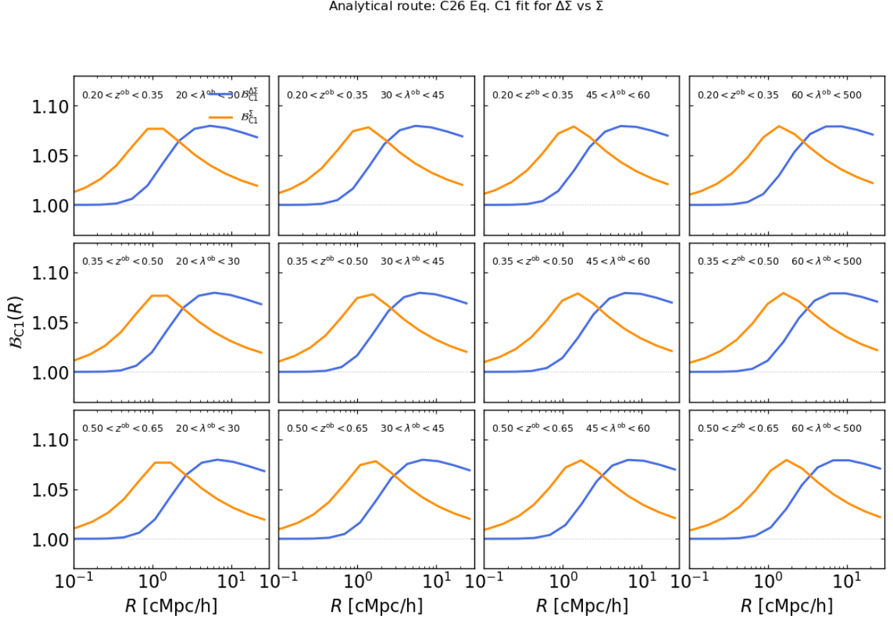
Figure 3: Analytical route: C26 Eq. C1 selection-bias ratio per (\lambda^{\text{ob}}, z^{\text{ob}}) bin on the DES Y1 grid. Blue: \mathcal{B}_{\text{sel},\text{C1}}^{\Delta\Sigma} (used in the data vector). Orange: \mathcal{B}_{\text{sel},\text{C1}}^{\Sigma} overlay. x -axis is comoving R in h^{-1} Mpc to match the C26 convention; y -axis is the bias factor.
