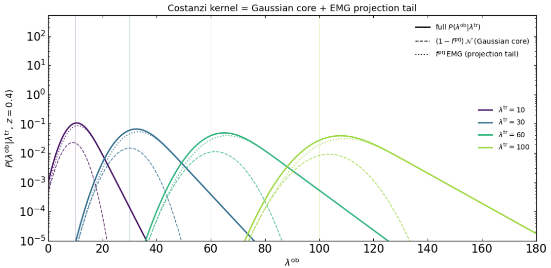
Figure 2: Decomposition of the C19 Eq. 6 kernel into its (1 - f_{\text{prj}})\mathcal{N} Gaussian core (dashed) and f_{\text{prj}} EMG projection tail (dotted) at z = 0.4 for four intrinsic richnesses \lambda^{\text{tr}} \in \{10, 30, 60, 100\} . The EMG tail rises with \lambda^{\text{tr}} and drives the optical-selection bias on the lensing data vector.
