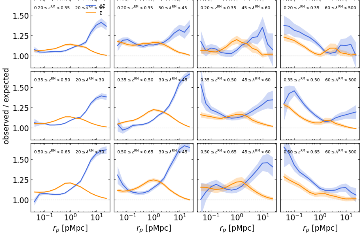
Figure 5: Empirical route: \mathcal{B}_{\text{sel}}^{\text{emp}}(R) per (\lambda^{\text{RM}}, z^{\text{RM}}) bin on the DES Y1 grid, with N_{\text{boot}} = 50 bootstrap bands. Blue: \Delta\Sigma ratio. Orange: \Sigma ratio (overlay). Reproduces Wu+2022 Fig. 2: the bell-shaped peak around R \sim 1 pMpc is the LSS-environment-driven selection bias signal.
