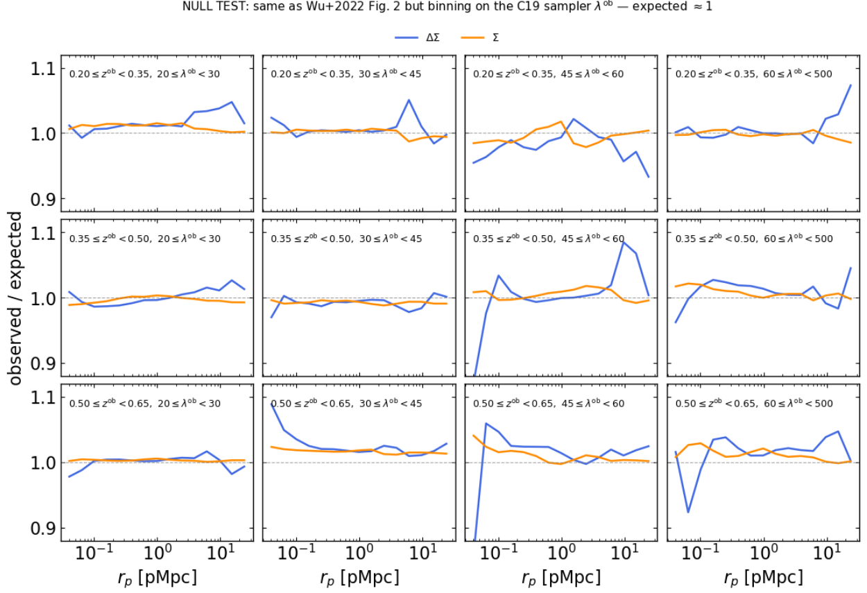
Figure 5: Null test: same Wu+22 panel grid but binning on the C19 sampler ( \lambda^{\text{ob}}, z^{\text{ob}} ) rather than the catalog ( \lambda^{\text{RM}}, z^{\text{RM}} ). The bell collapses to \approx 1 across all bins, confirming the R \sim 1 pMpc peak in Fig. 4 is genuinely LSS-driven.
