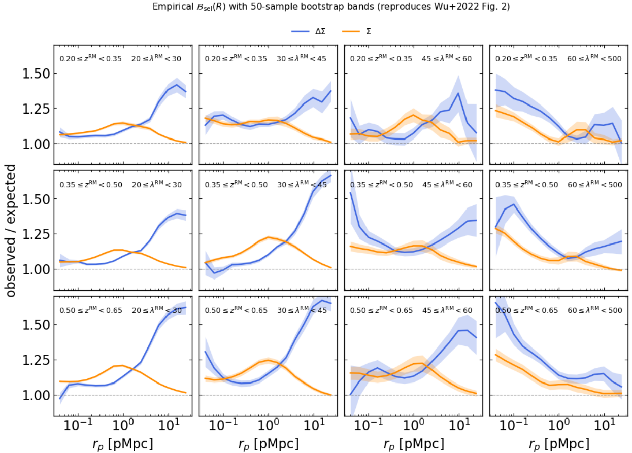
Figure 4: Empirical route: \mathcal{B}_{\text{sel}}^{\text{emp}}(R) per (\lambda^{\text{RM}}, z^{\text{RM}}) bin on the DES Y1 grid, with N_{\text{boot}} = 50 bootstrap bands. Blue: \Delta\Sigma ratio. Orange: \Sigma ratio (overlay). Reproduces Wu+2022 Fig. 2: the bell-shaped peak around R \sim 1 pMpc is the LSS-environment-driven selection bias signal.
