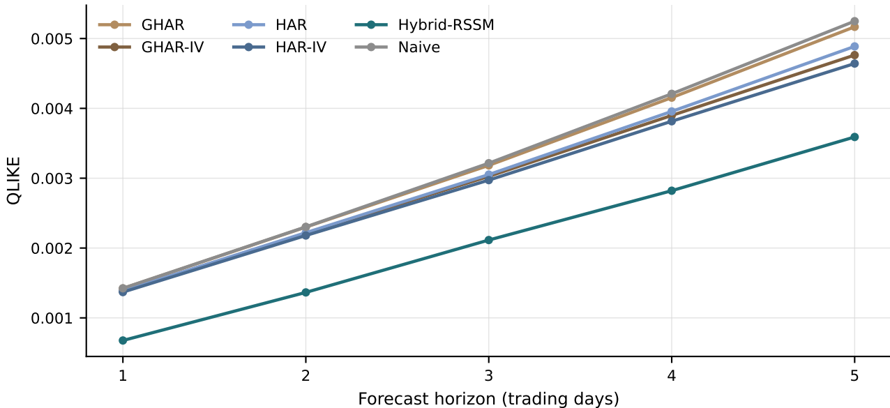
Out-of-sample QLIKE by forecast horizon
