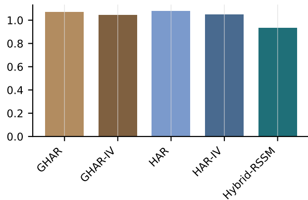
Cross-sectional correlation RMSE
