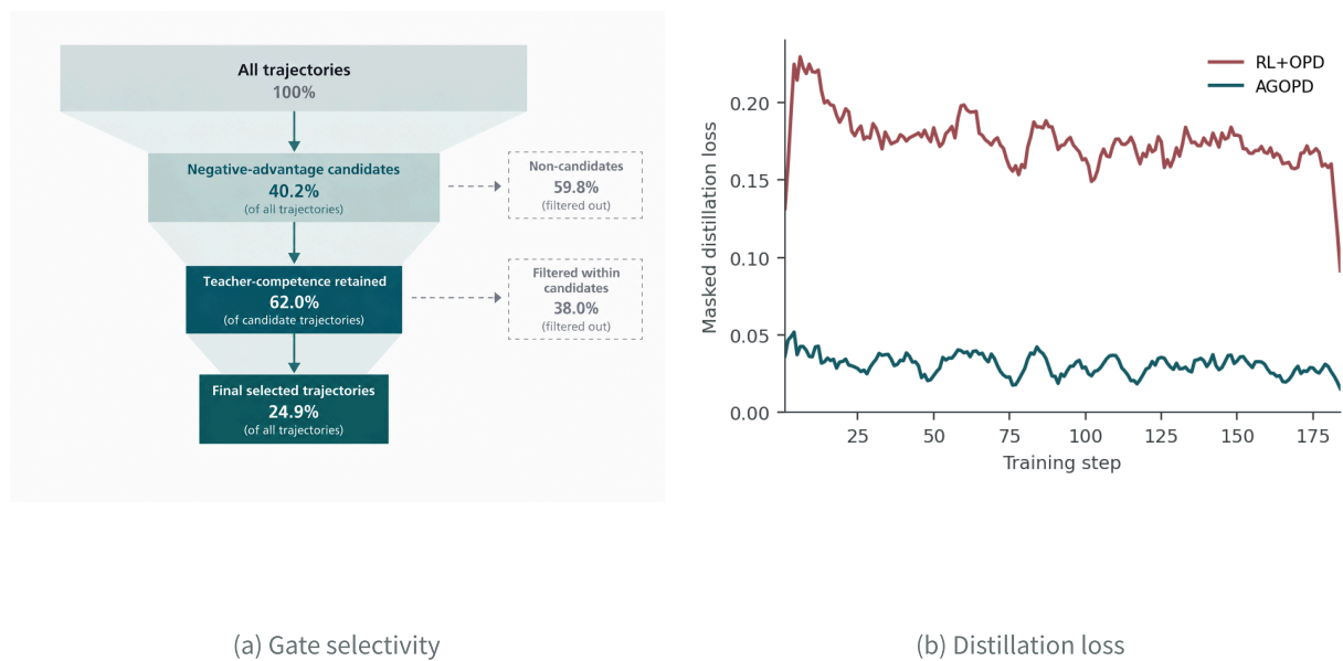
Figure 5 • Gating dynamics and distillation scope.(a) Report the proportion of negative dominant candidates after aggregation of 180 training steps, and the proportion of teachers who are qualified and retained based on the candidate set.(b) Seven-step moving average of the distillation loss recorded in the training log; the distillation loss is affected by the mask, trajectory weight and sample difficulty at the same time, and is only used as a training diagnostic quantity and not as an independent estimate of the gradient scope.
