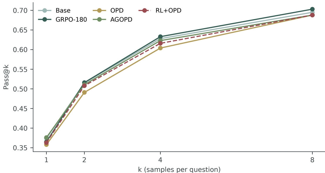
Pass@k across methods
