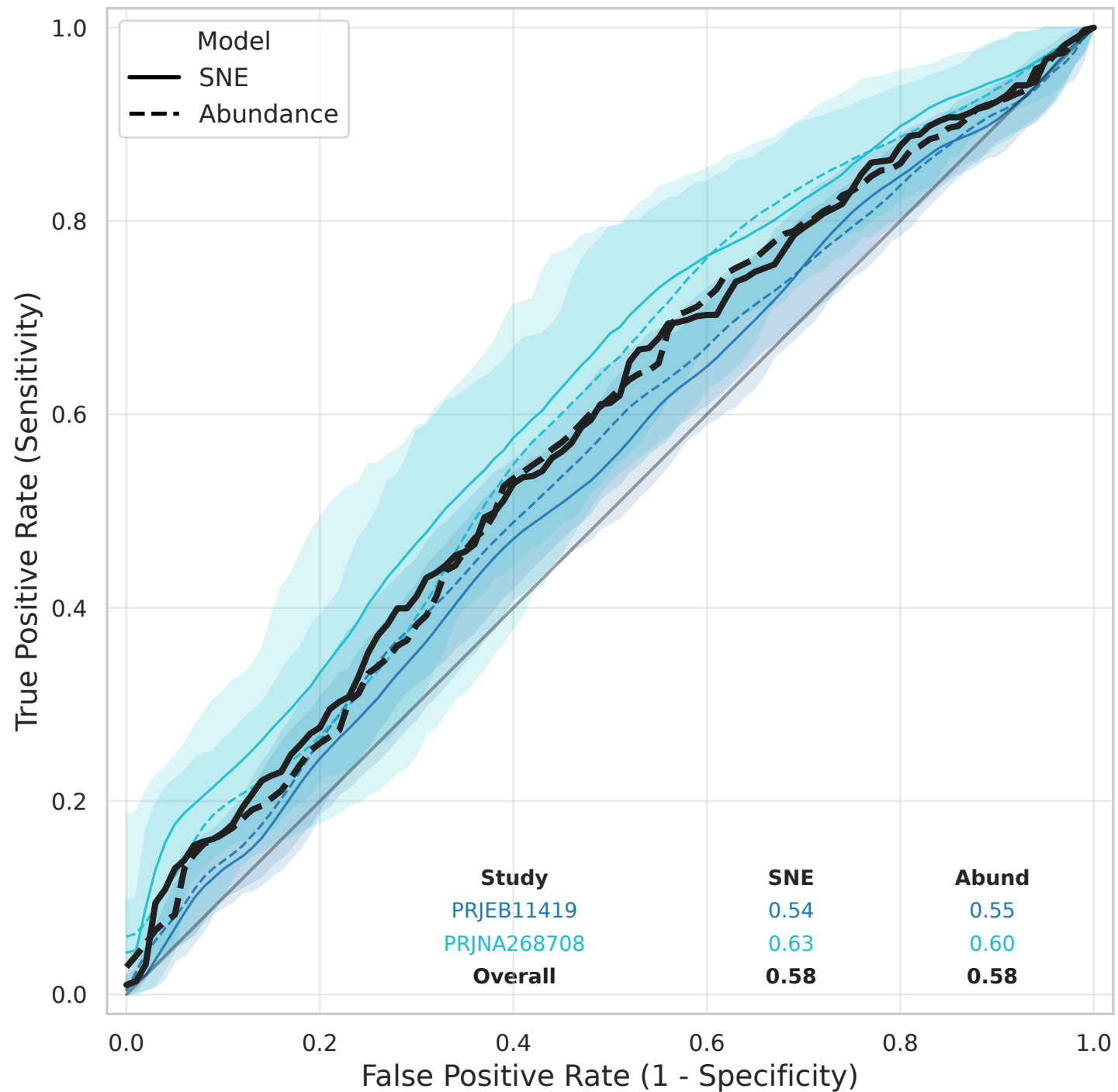
ROC Curves with 95% CI for IBS
