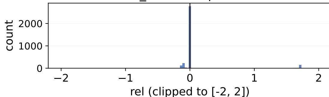
trait_monomorphization
