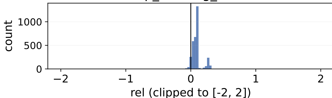
loop_hoisting_bench
