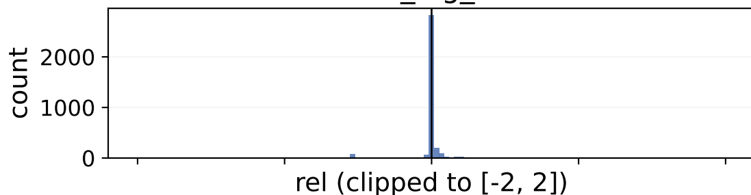
branch_cfg_bench
