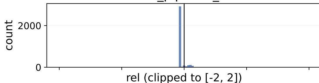
iterator_pipeline_bench
