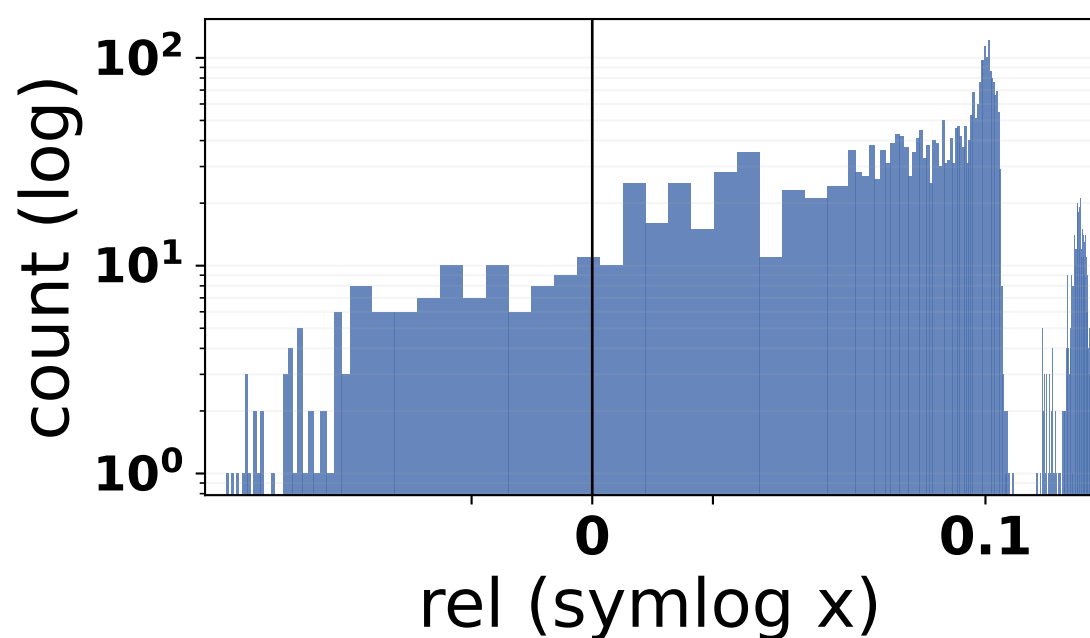
loop_hoisting_bench
