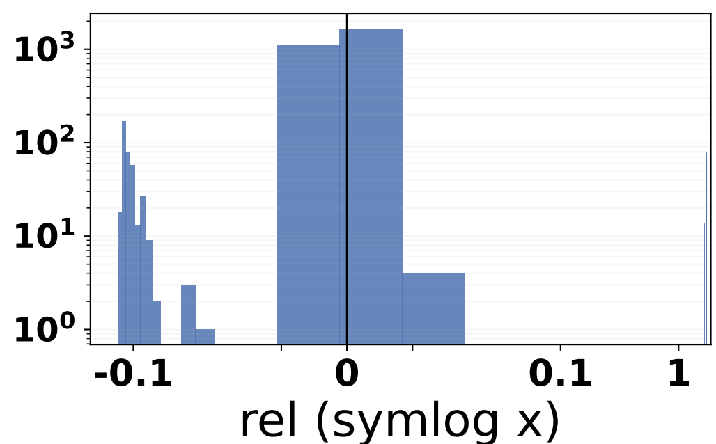
trait_monomorphization
