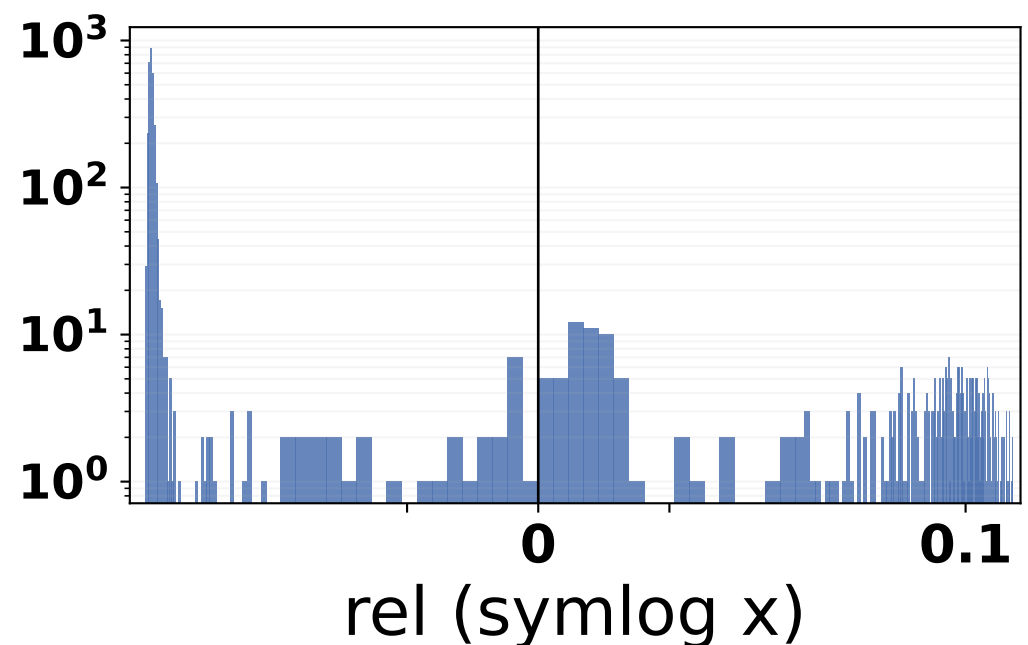
trait_monomorphization
