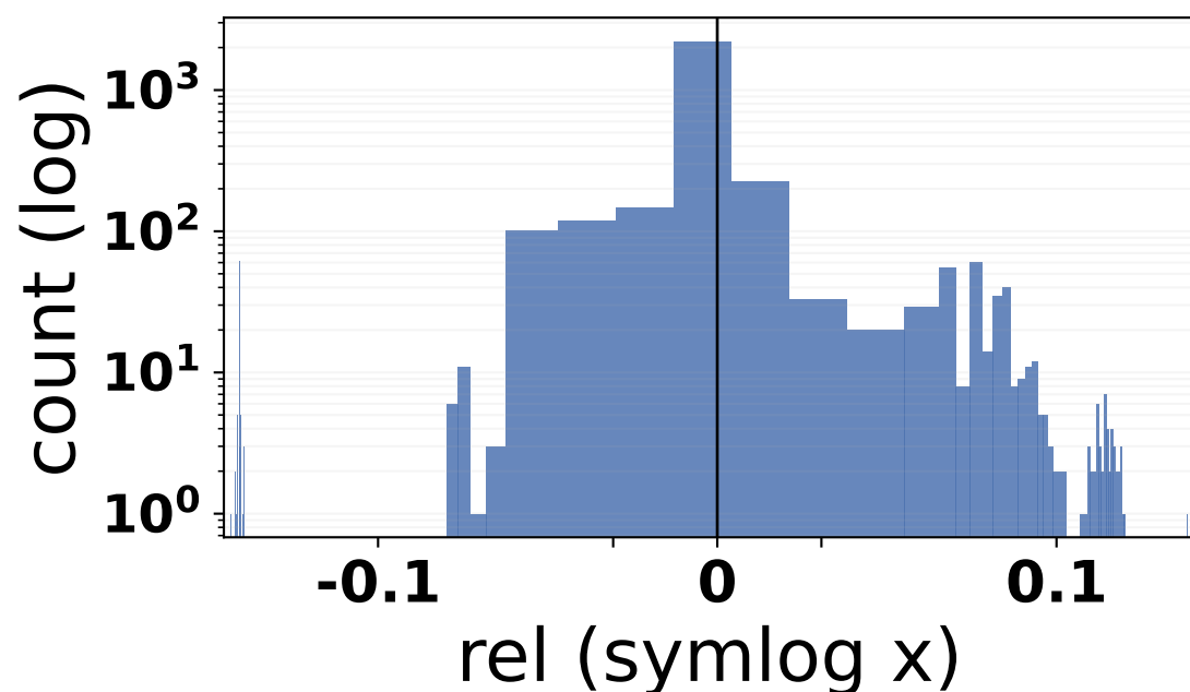
loop_hoisting_bench
