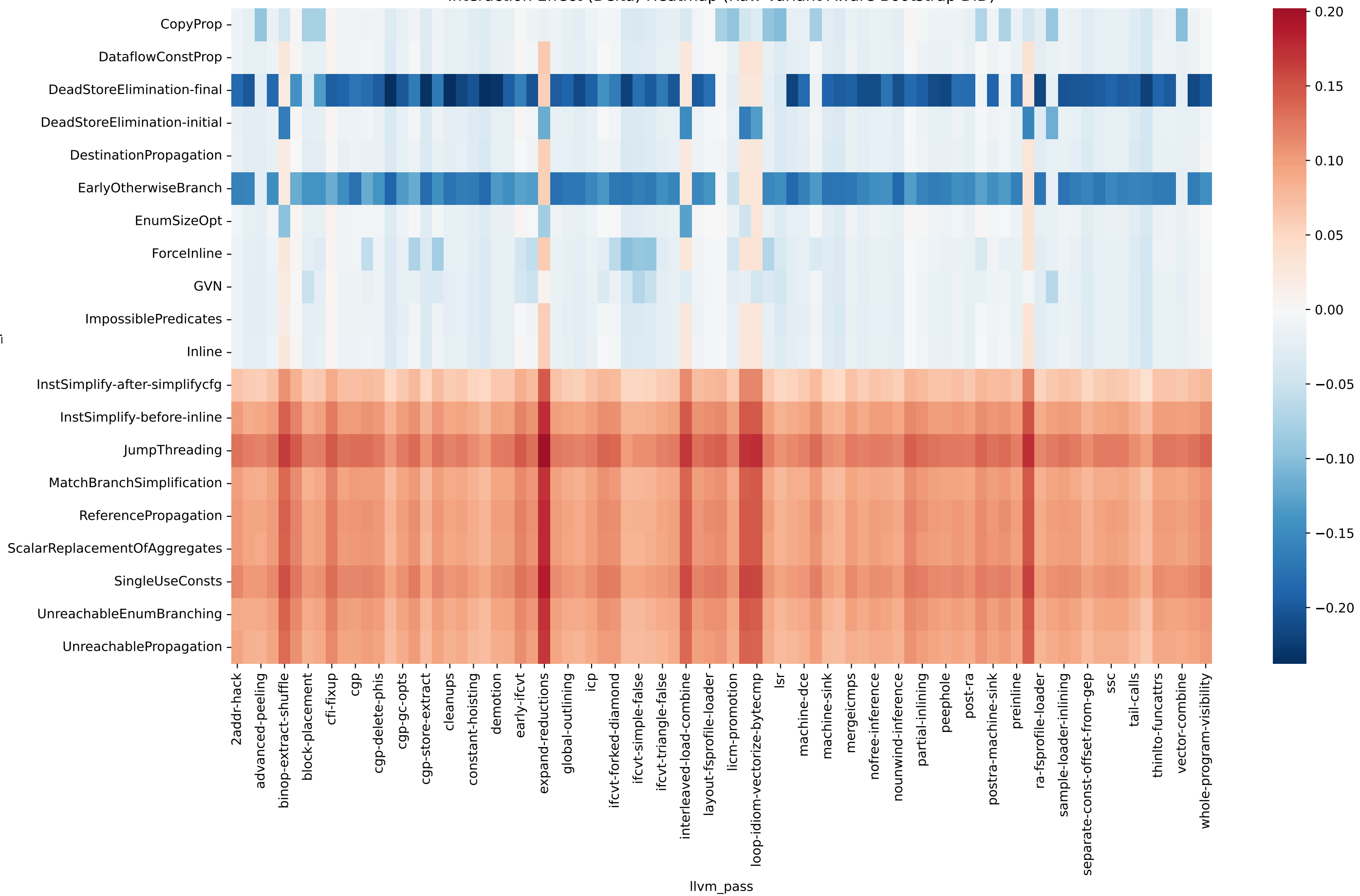
Interaction Effect (Delta) Heatmap (Raw Variant-Aware Bootstrap DiD)
