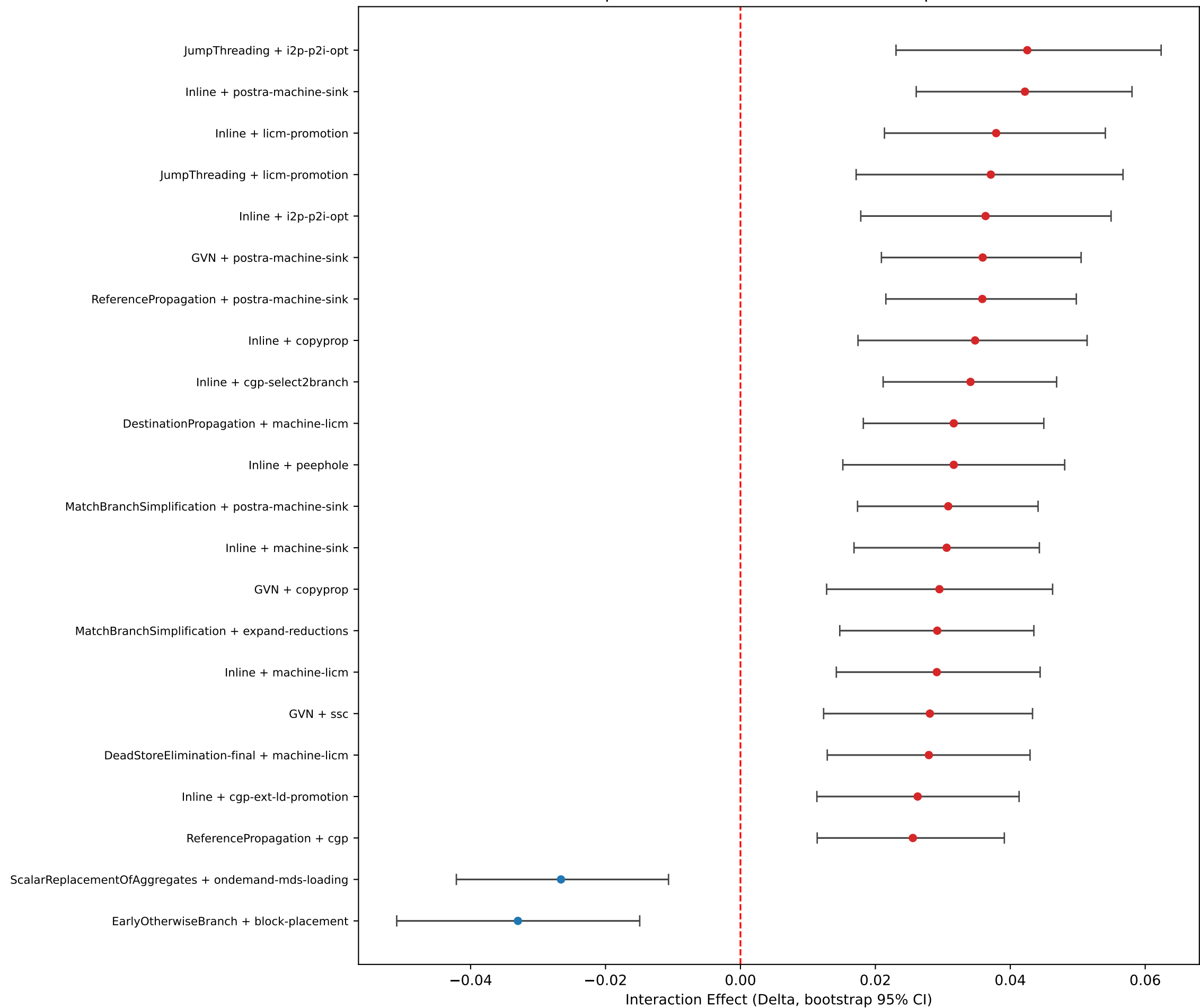
Top Interactions from Raw-Run Bootstrap DiD
