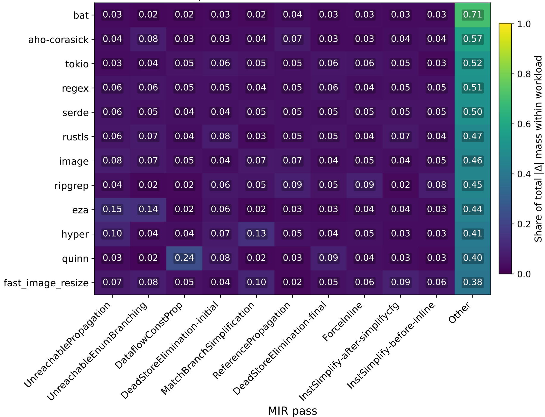
MIR-pass dominance across workloads
