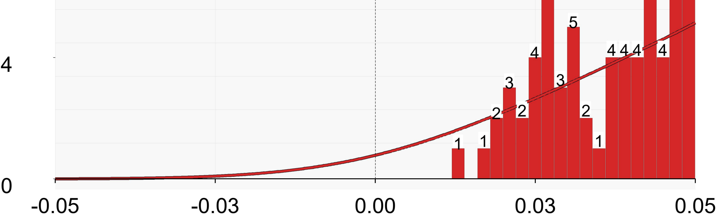
(b) Positive interaction (n=1095)
