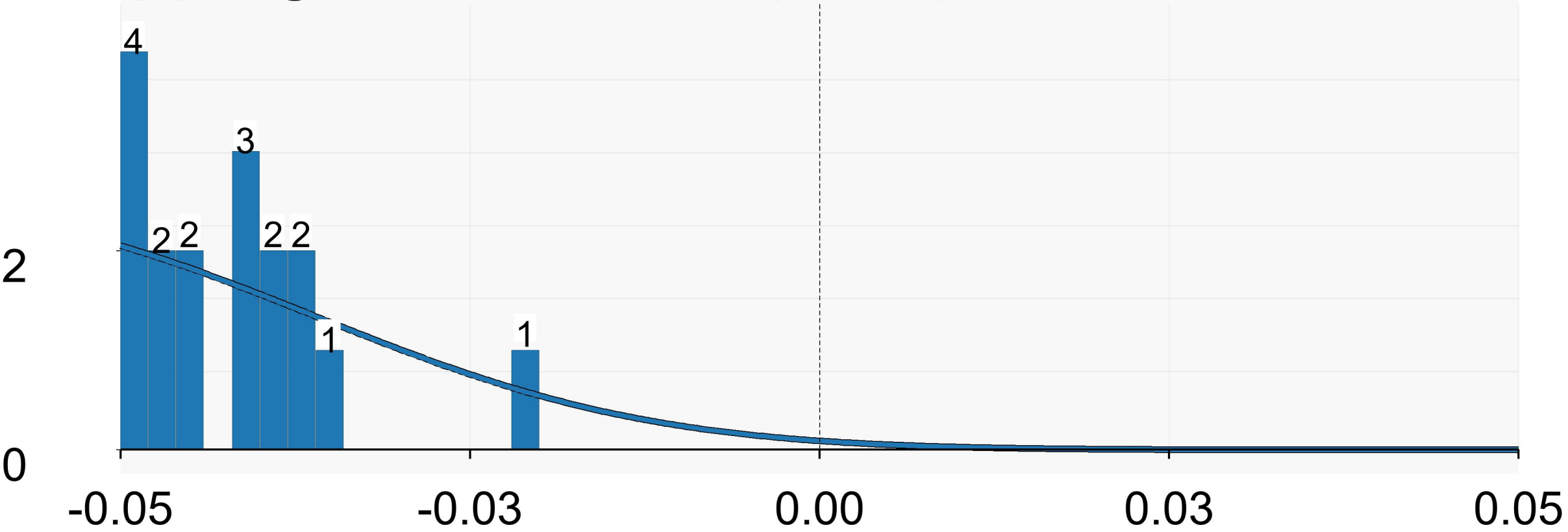
(a) Negative interaction (n=335)
