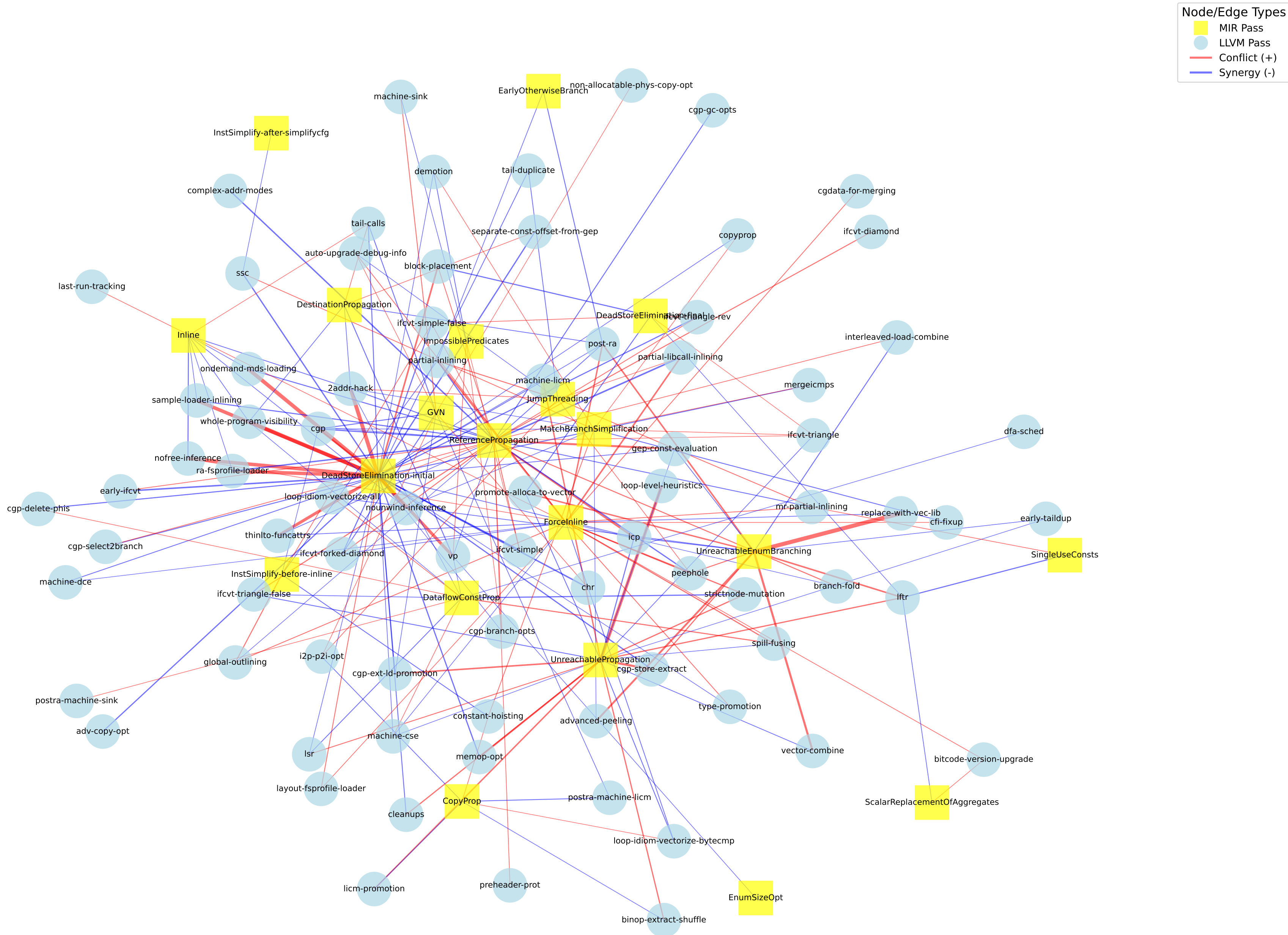
hyper (anova) Cross-Level Coupling Graph Square=MIR, Circle=LLVM | Red=Conflict(+), Blue=Synergy(-)
