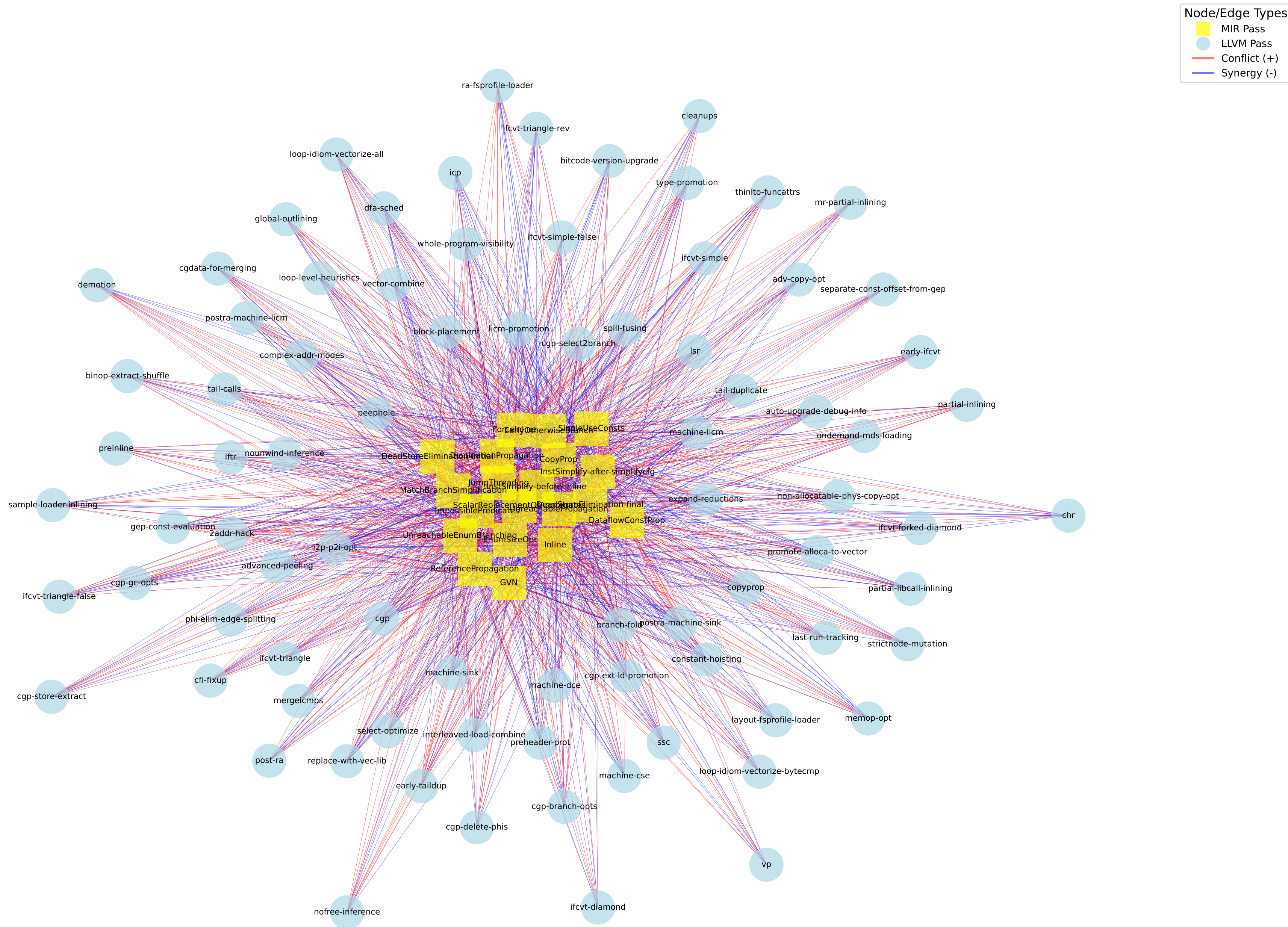
regex (lasso) Cross-Level Coupling Graph Square=MIR, Circle=LLVM | Red=Conflict(+), Blue=Synergy(-)
