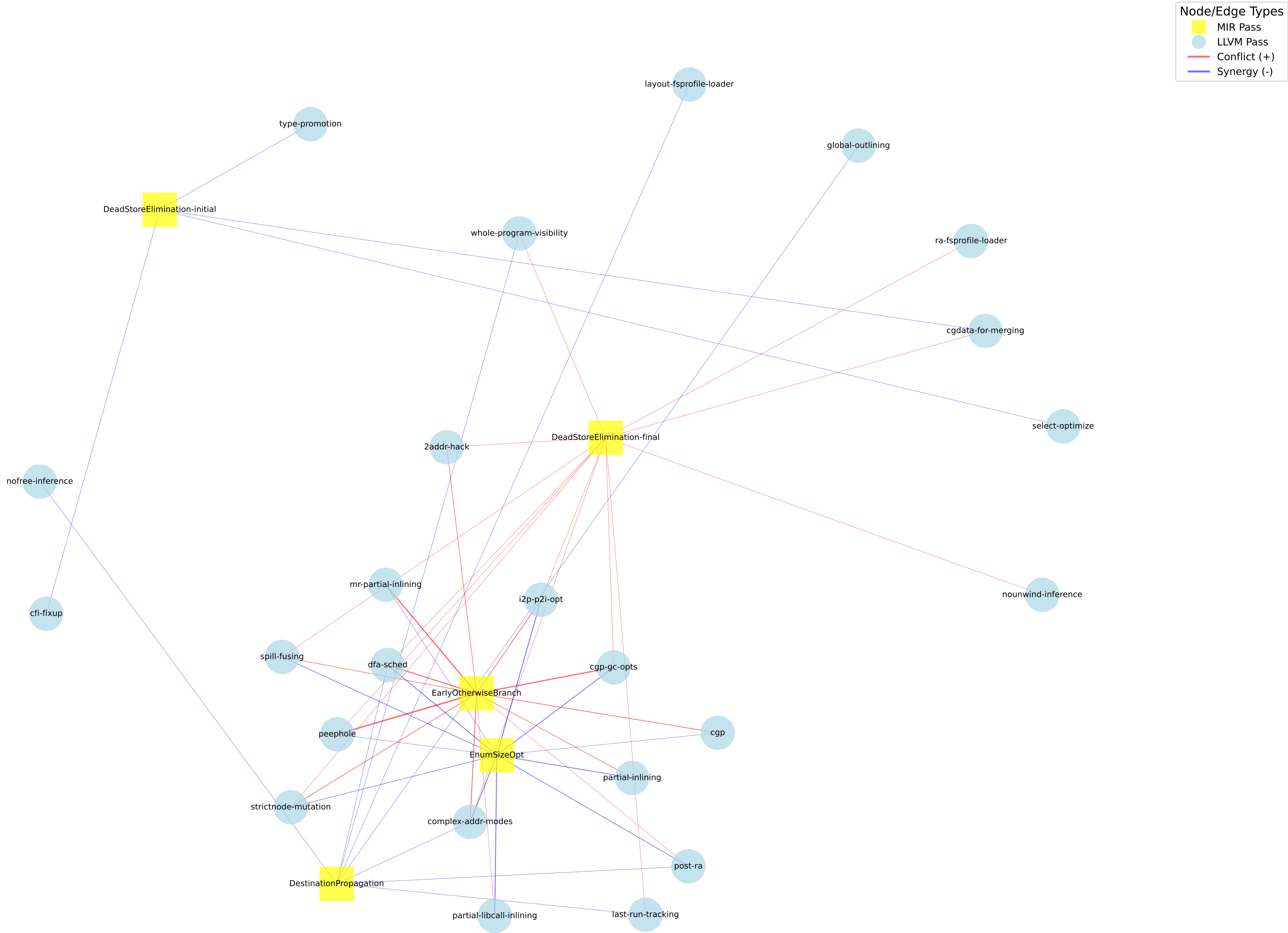
ripgrep (lasso) Cross-Level Coupling Graph Square=MIR, Circle=LLVM | Red=Conflict(+), Blue=Synergy(-)
