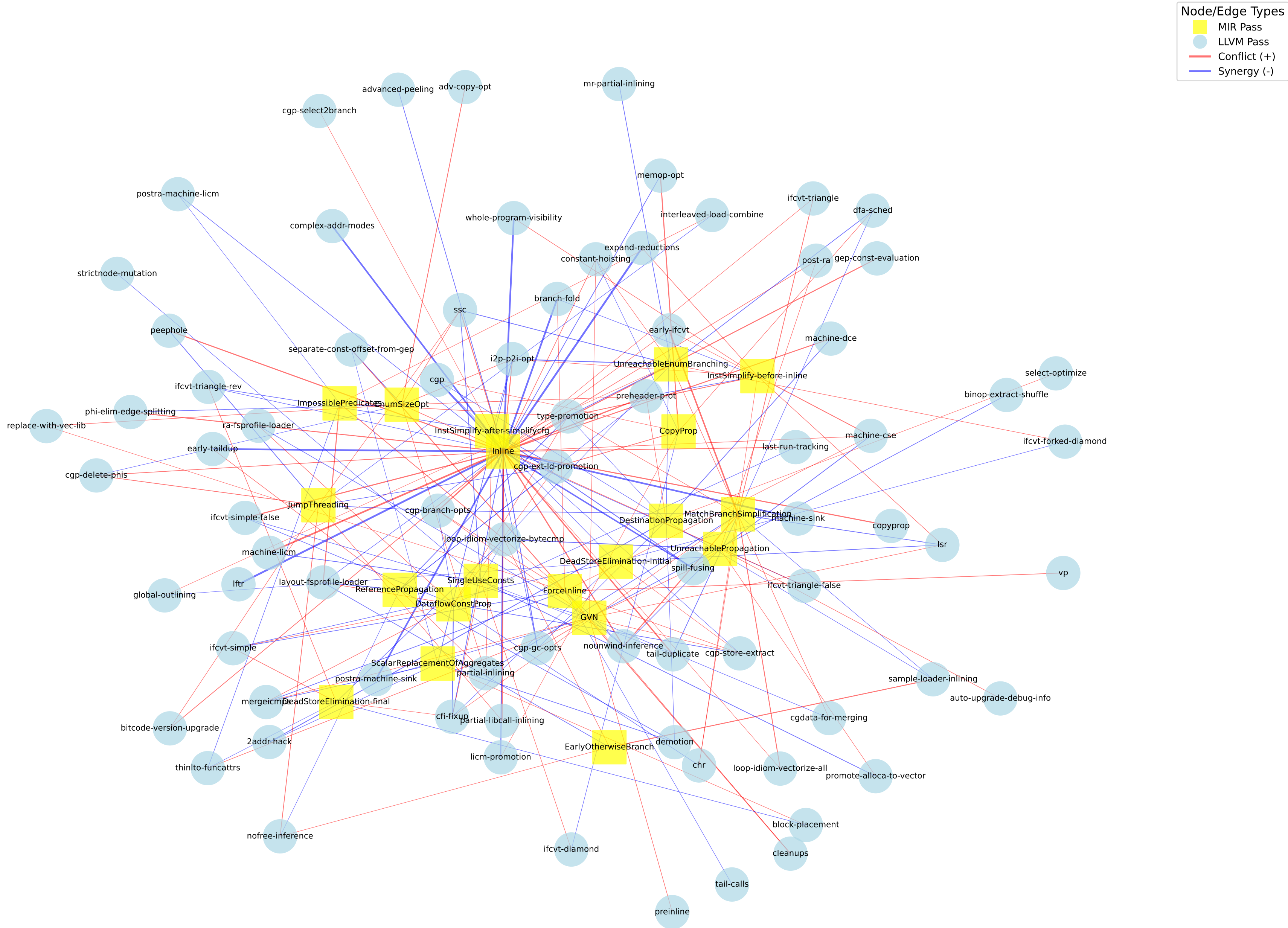
tokio (anova) Cross-Level Coupling Graph Square=MIR, Circle=LLVM | Red=Conflict(+), Blue=Synergy(-)
