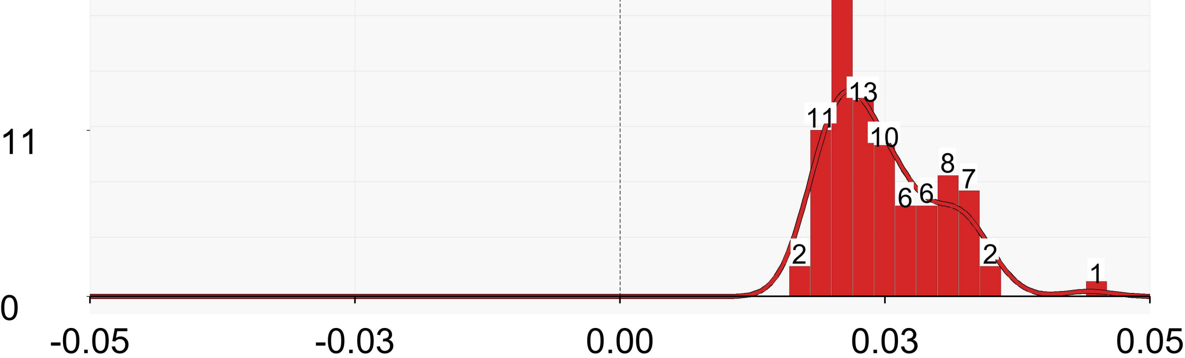
(b) Positive interaction (n=86)
