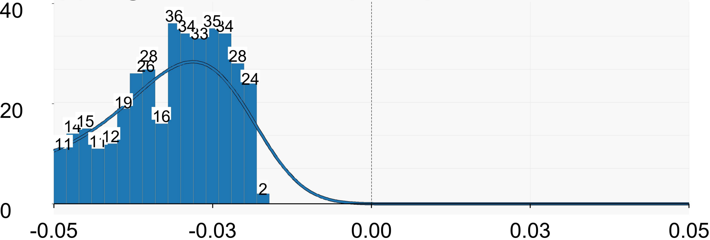
(a) Negative interaction (n=491)
