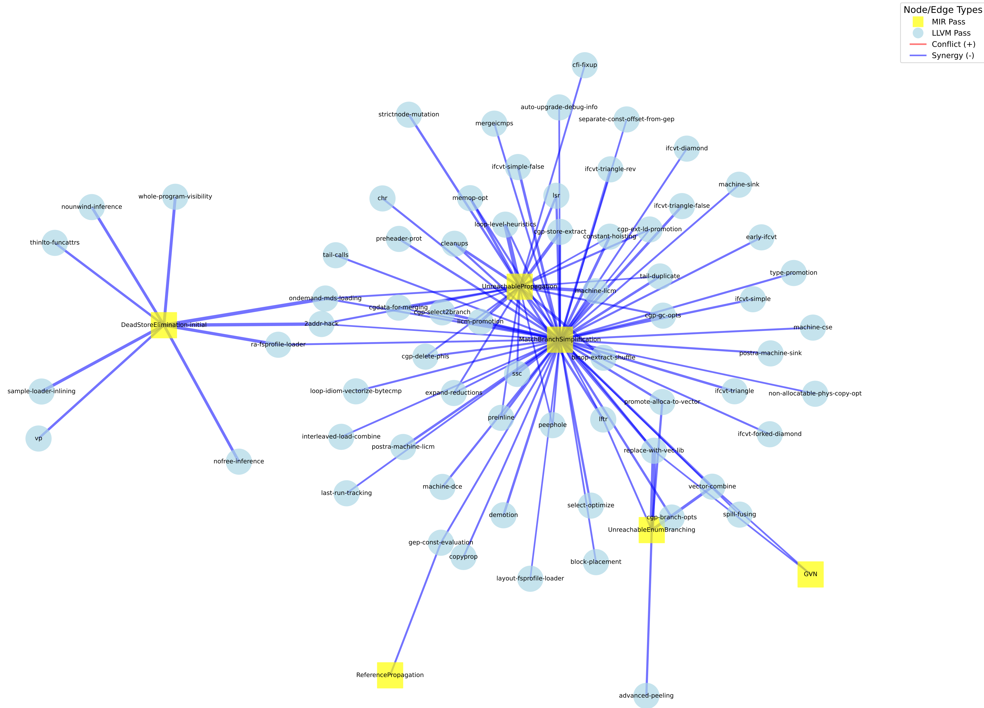
Cross-Level Coupling Graph (Lasso on Raw Runs) Square=MIR, Circle=LLVM | Red=Conflict(+), Blue=Synergy(-)
