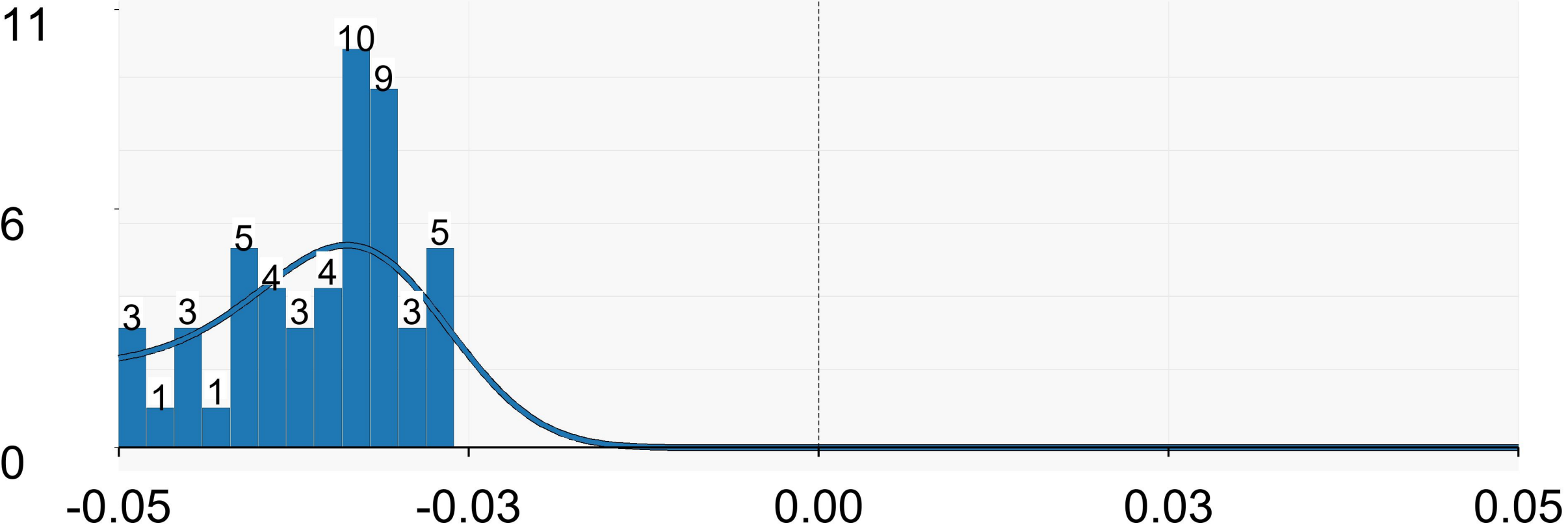
(a) Negative interaction (n=67)
