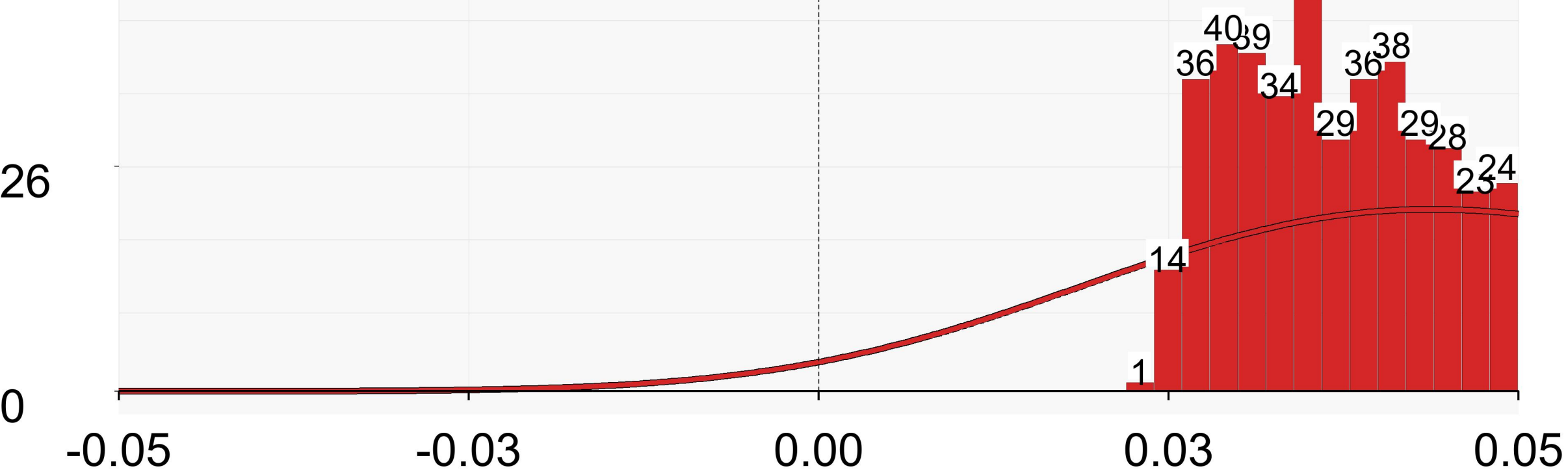
(b) Positive interaction (n=837)
