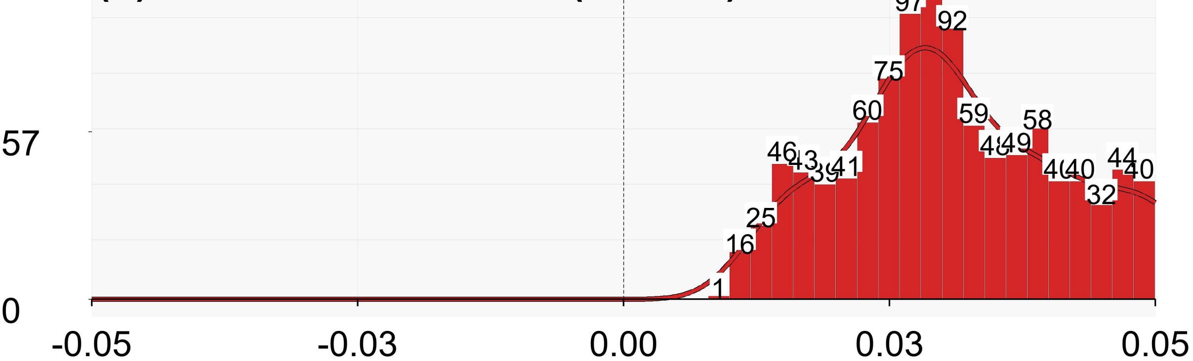
(b) Positive interaction (n=1164)
