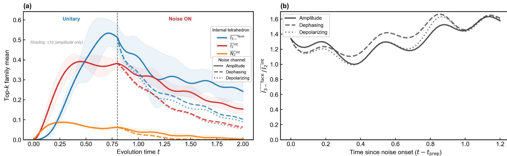
Noise robustness in the 5-qubit tetrahedral extension (top-k prepared families, g_E = 0.2 , t_{\text{prep}} = 0.8 , \gamma = 0.2 , k = 10 )
