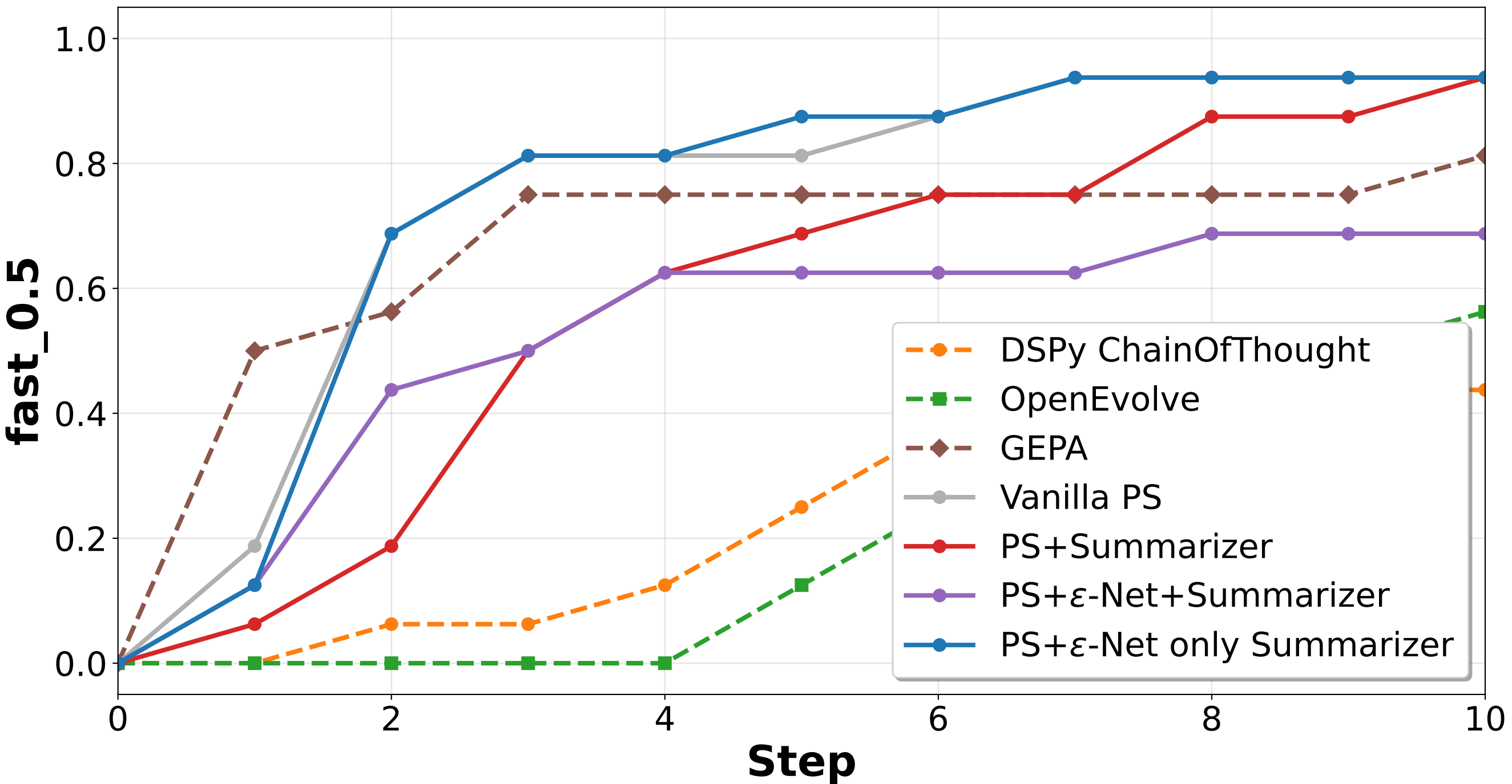
KernelBench fast_0.5 Over Steps
