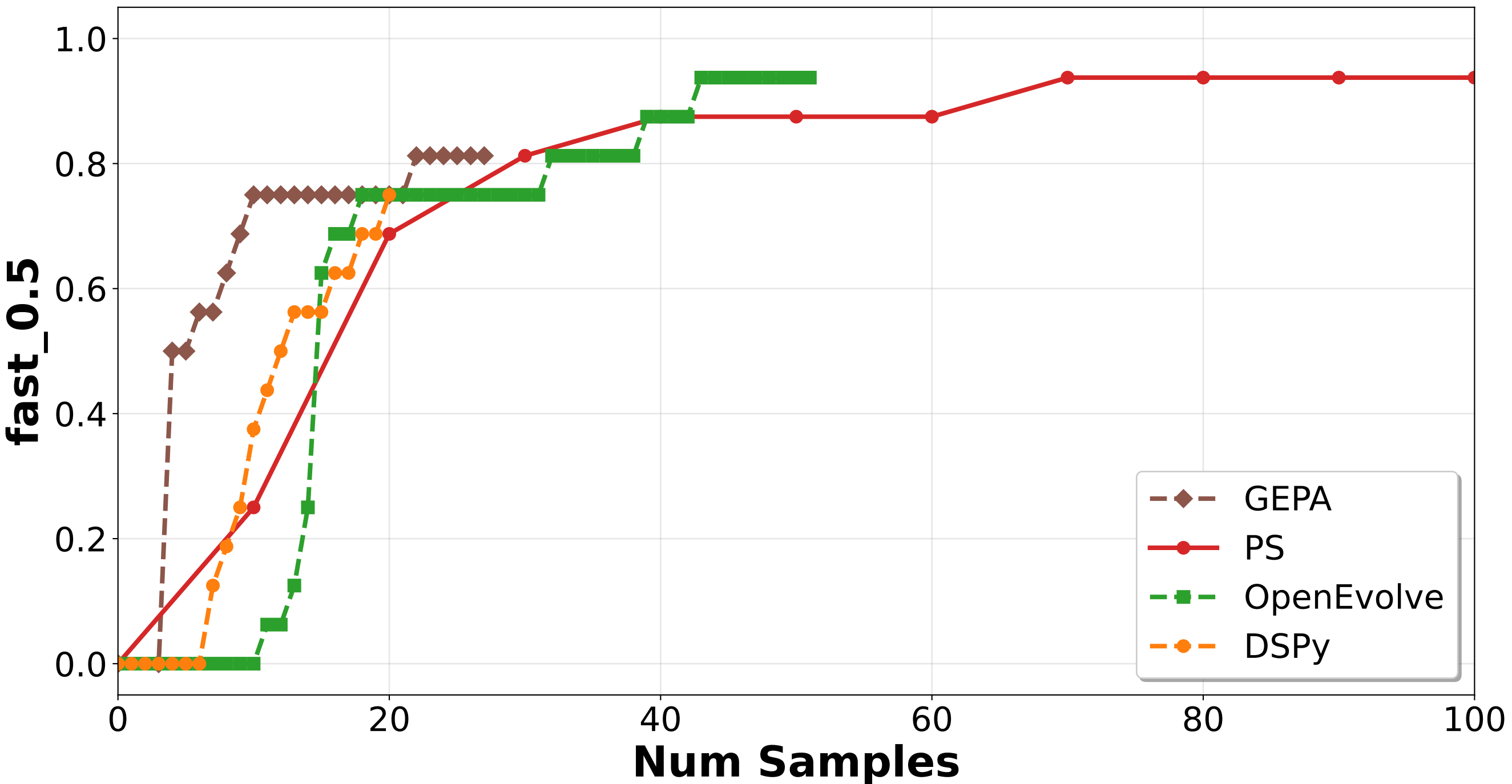
KernelBench fast_0.5 Over Num Samples
