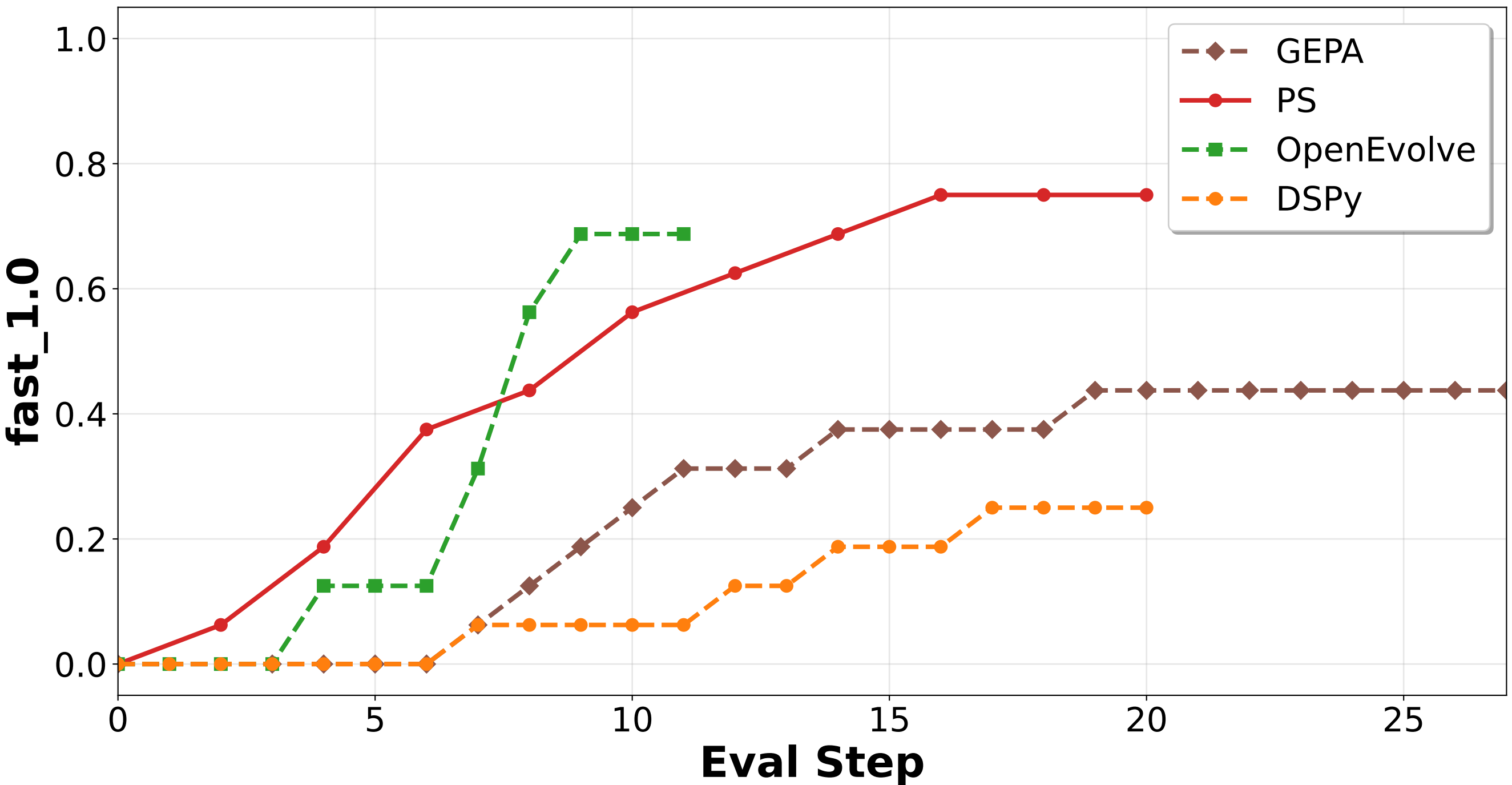
KernelBench fast_1.0 Over Eval Step
