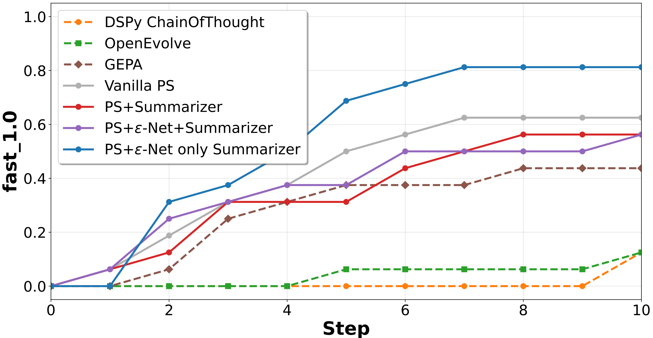
KernelBench fast_1.0 Over Steps
