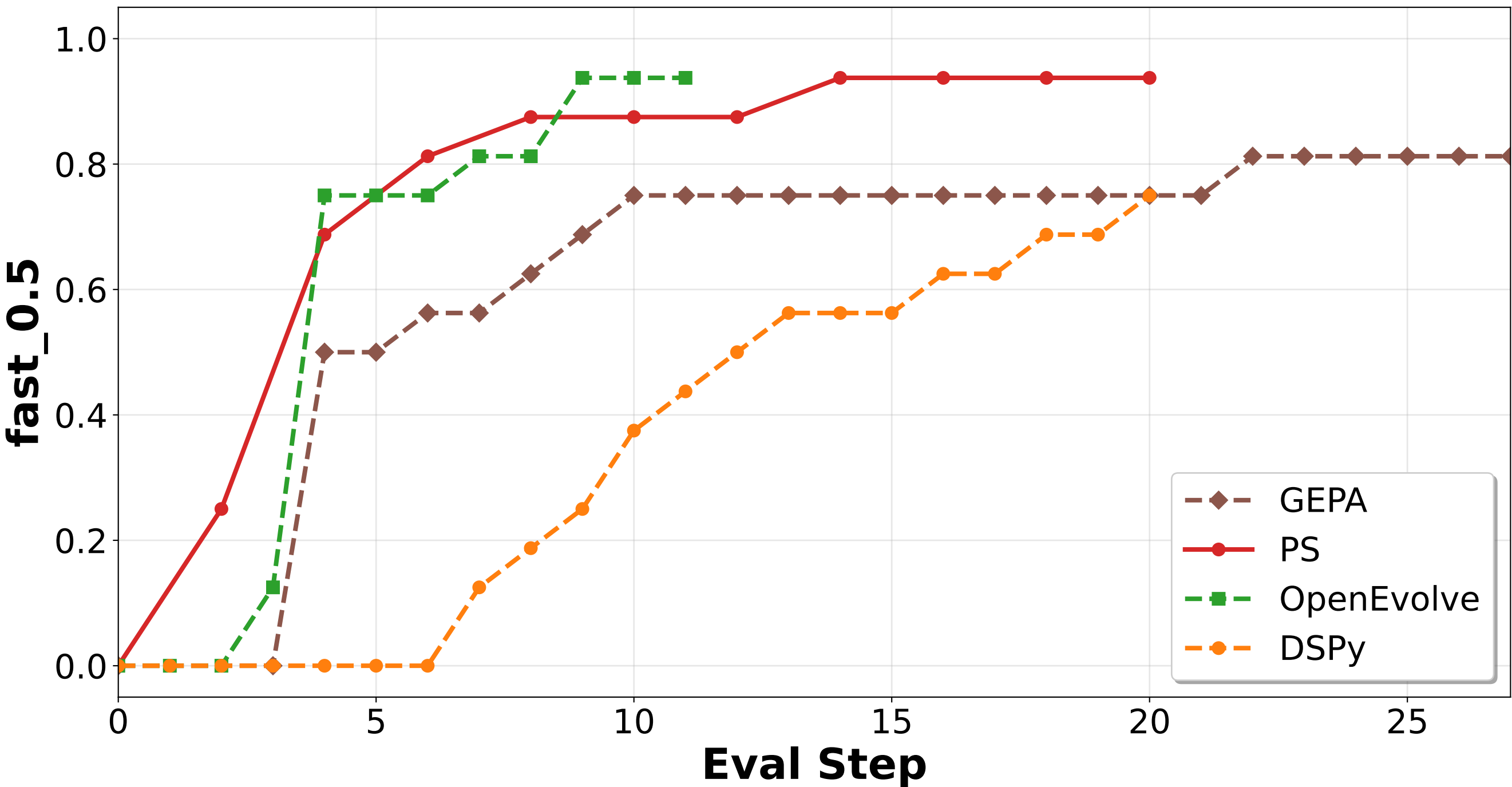
KernelBench fast_0.5 Over Eval Step
