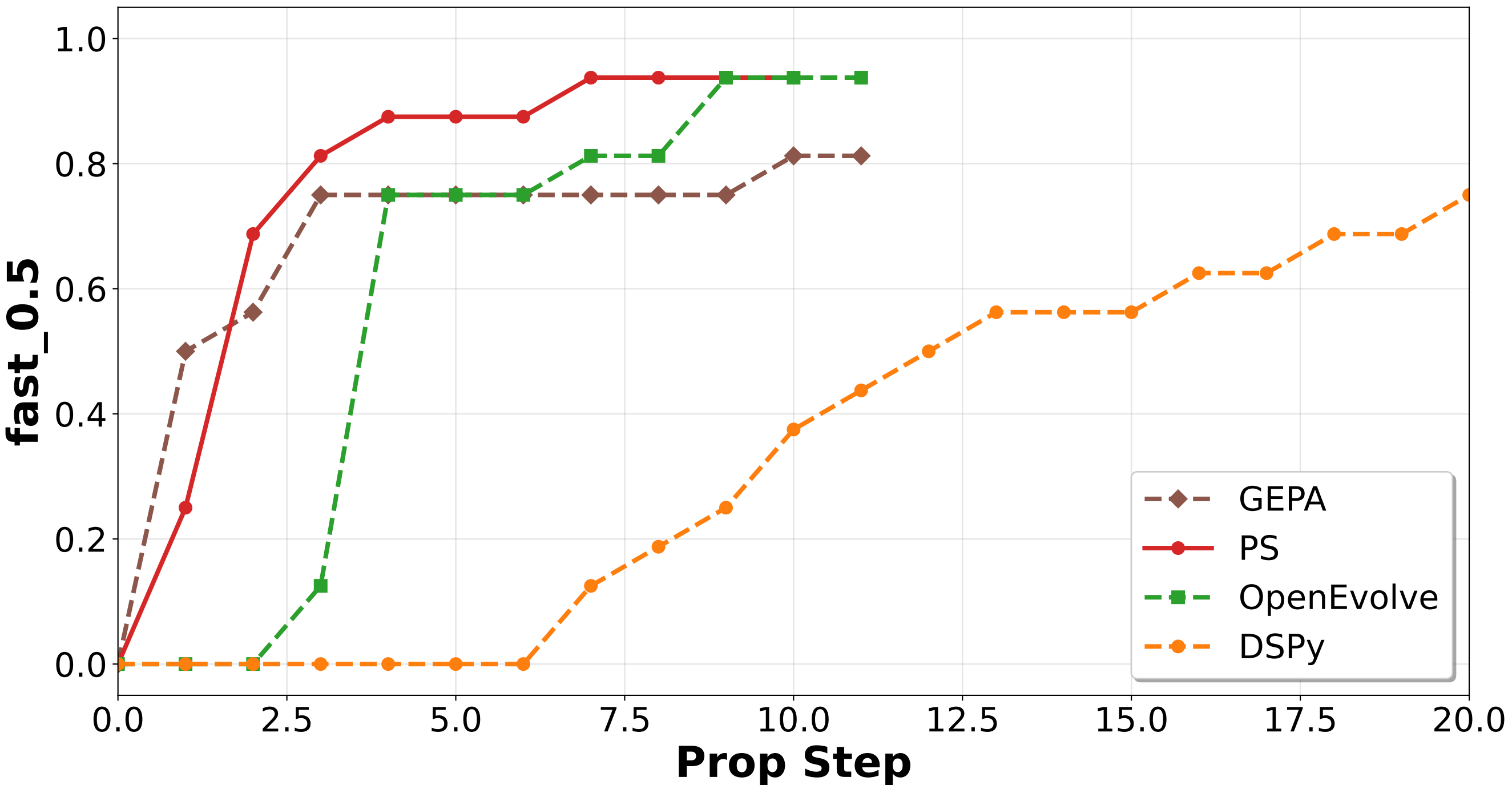
KernelBench fast_0.5 Over Prop Step
