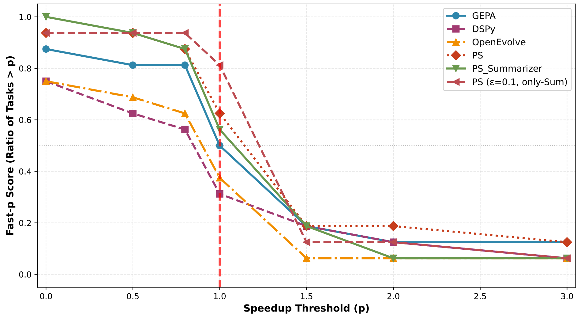
KernelBench: Fast-p Performance Comparison ( p \in [0, 3] )
