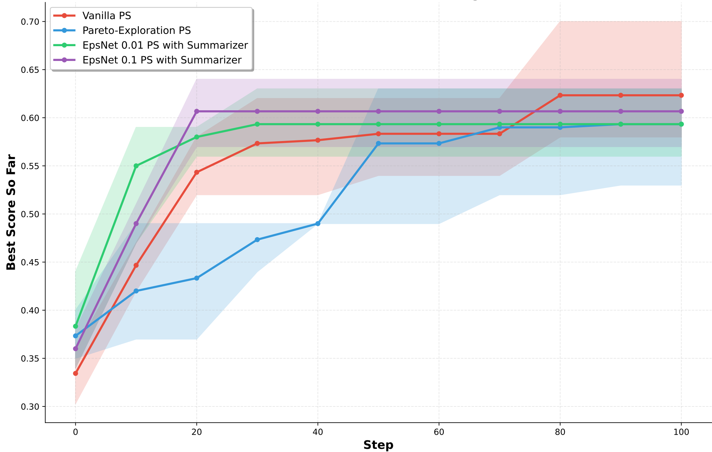
Cumulative Best Scores Across Algorithms
