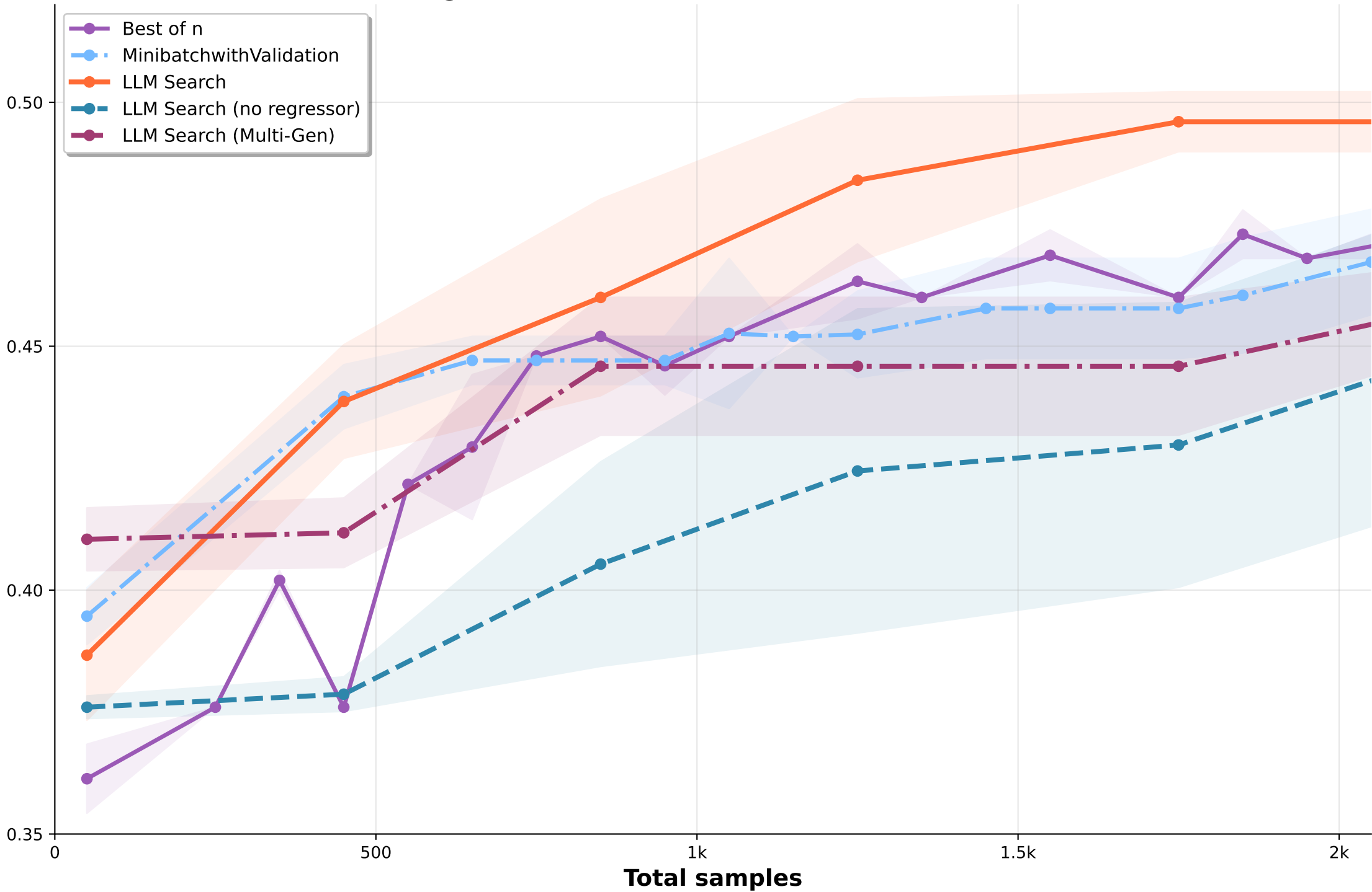
Highest score so far with Standard Error
