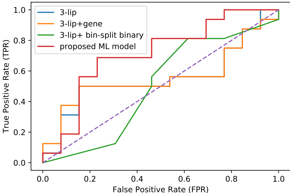
Receiver Operating Characteristic (ROC) Curve
