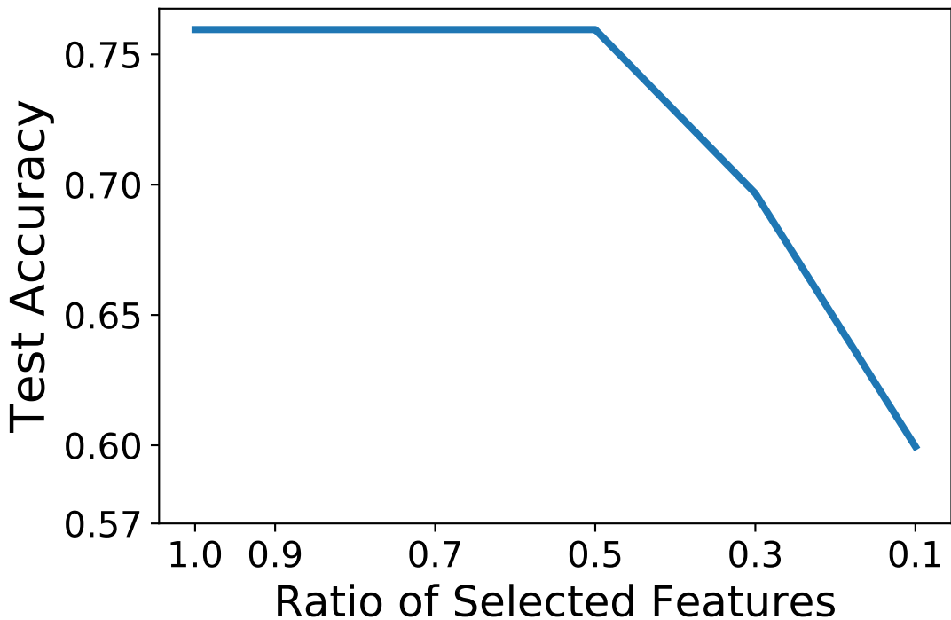
mHSPC:Survival
