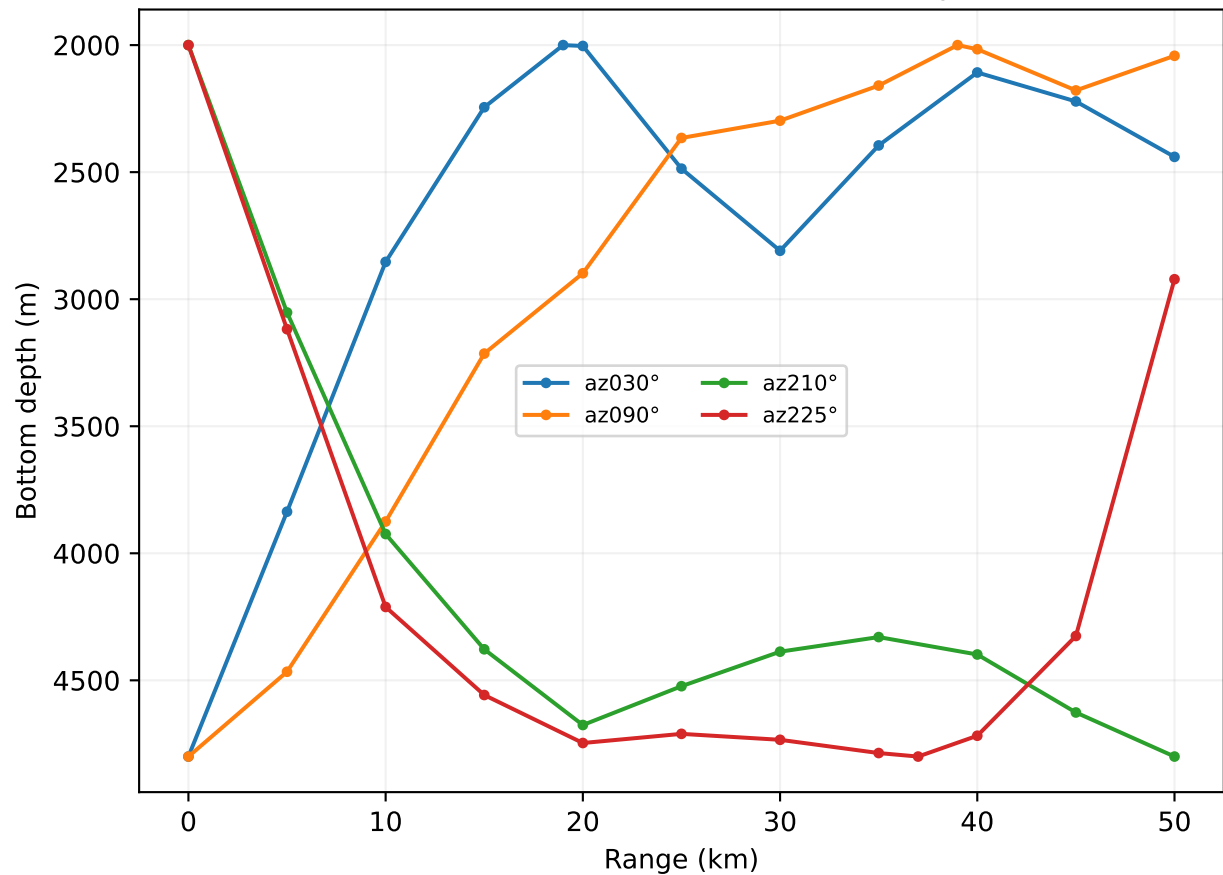
Four screened low-dimensional GEBCO profiles
