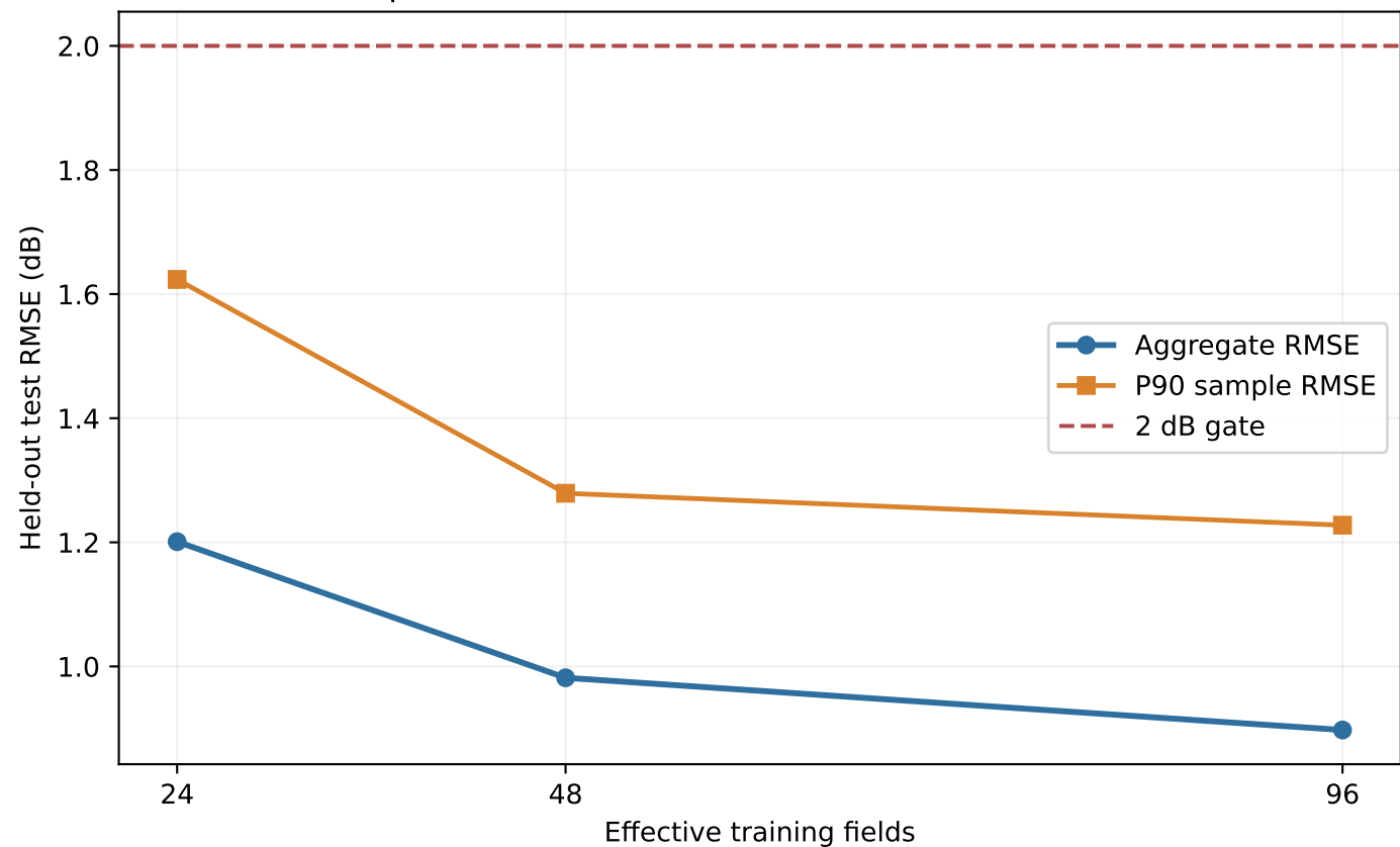
Grouped data-size ablation on the same sealed test set
