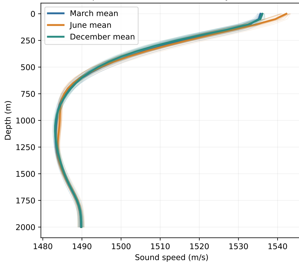
Three representative WOA23 monthly SSP families
