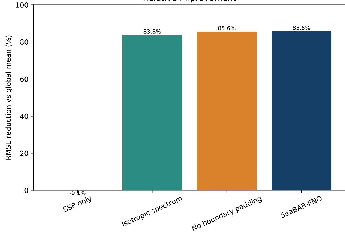
Relative improvement
