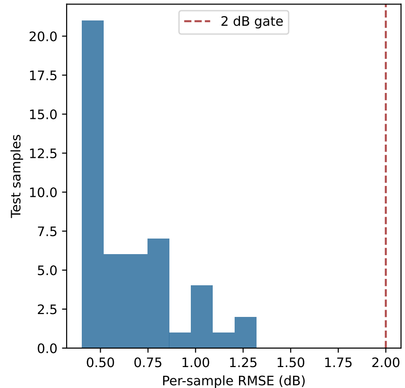
Held-out sample distribution
