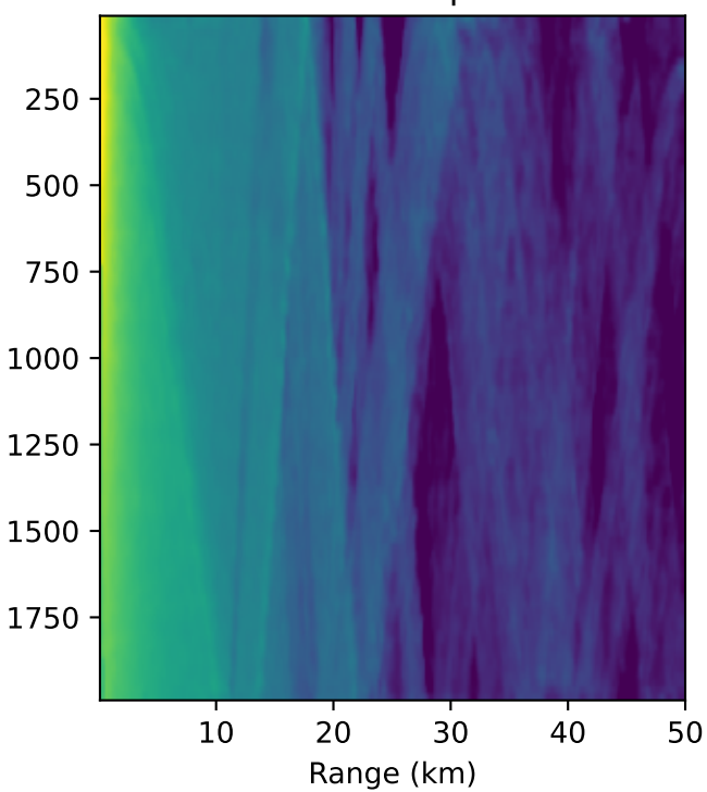
SourceBAR-FNO prediction
