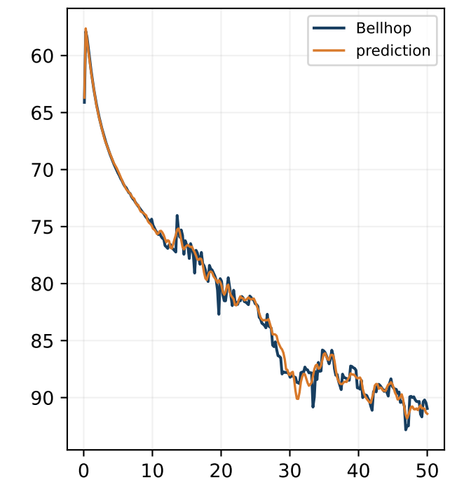
1000 m receiver slice; field RMSE 1.09 dB
