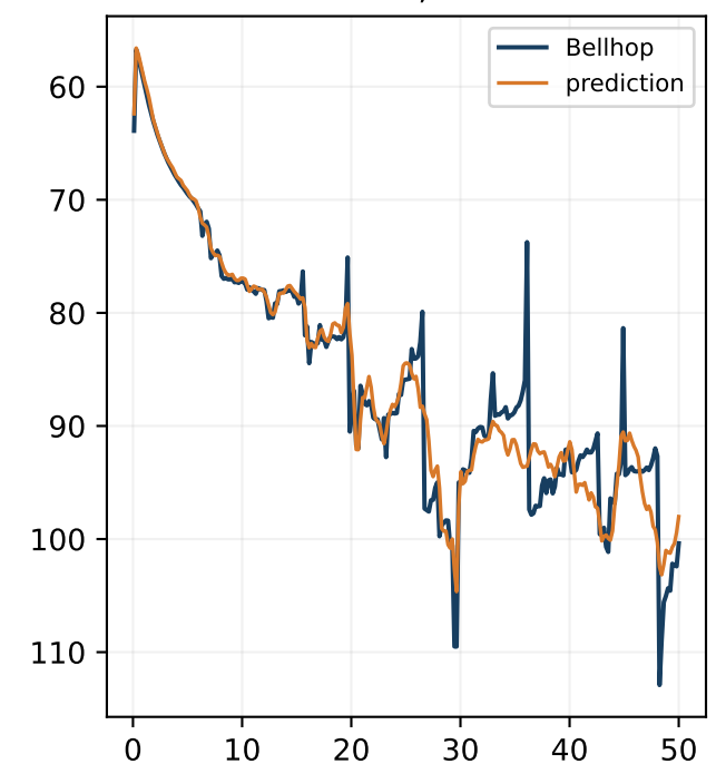
1000 m receiver slice; field RMSE 2.79 dB
