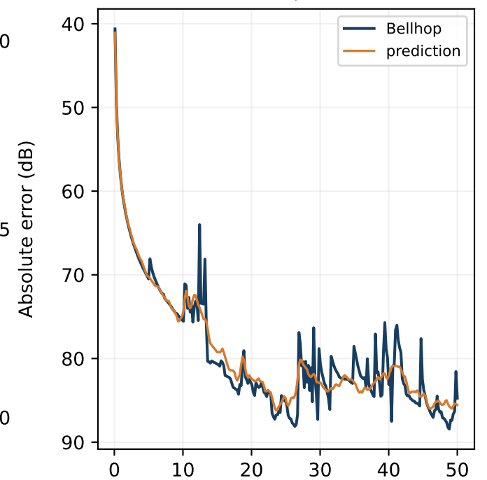
1000 m receiver slice; field RMSE 1.53 dB
