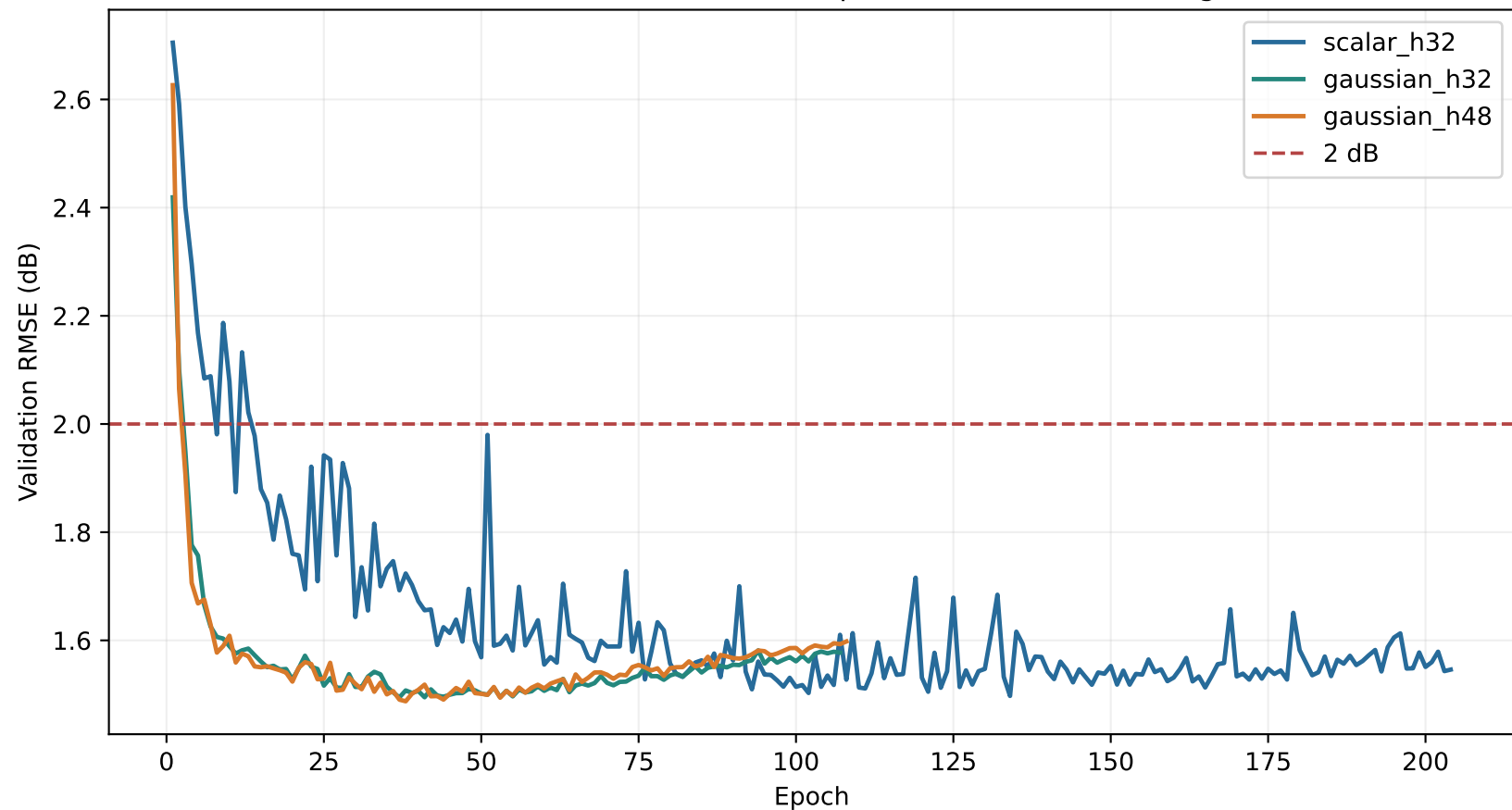
Model selection on source depths absent from training
