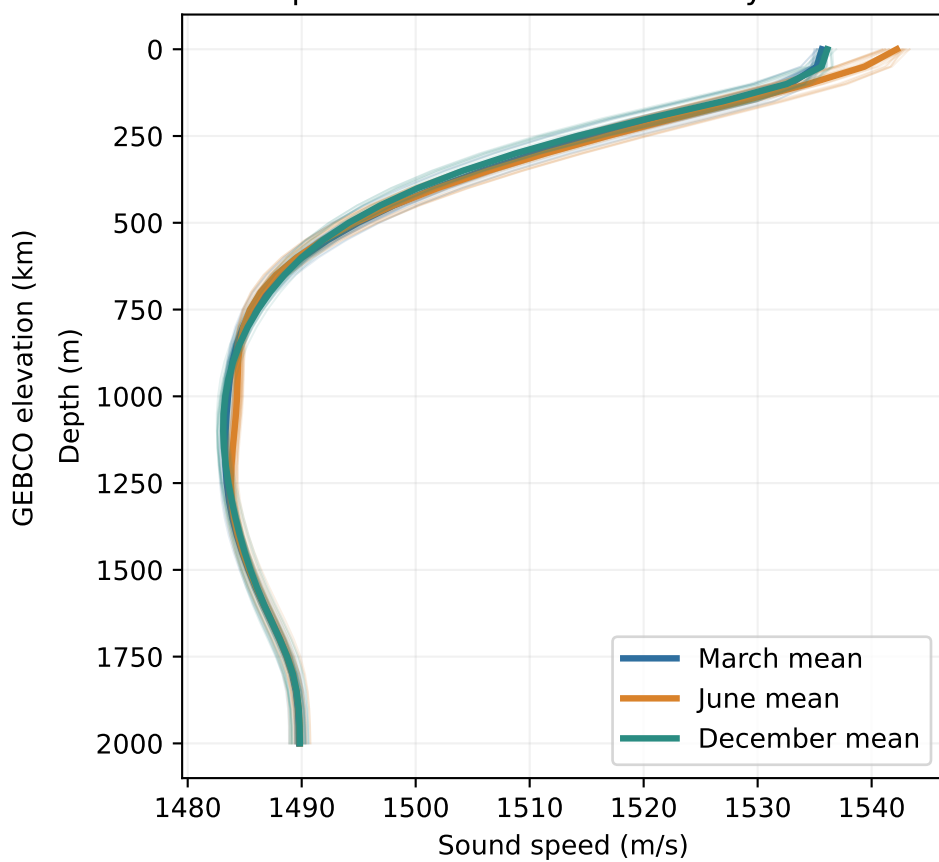
Three representative WOA23 monthly SSP families
