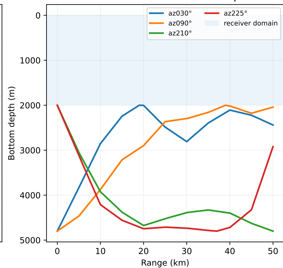
Screened low-dimensional bottom profiles
