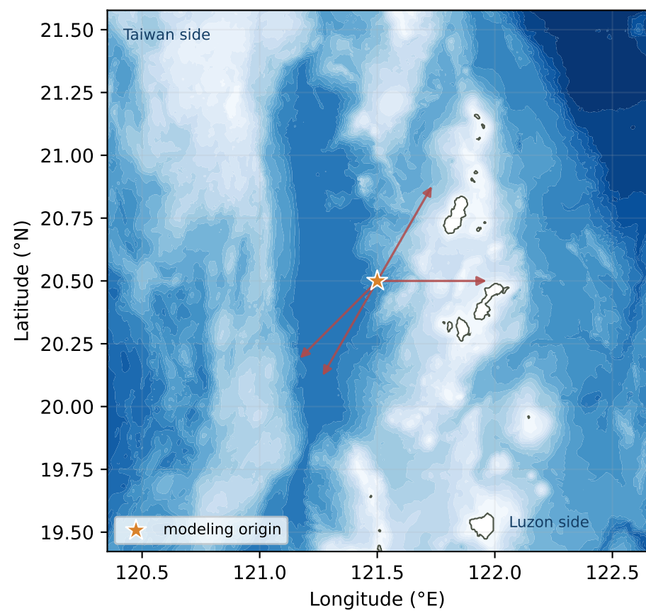
Bashi Channel location and four 50 km directions
