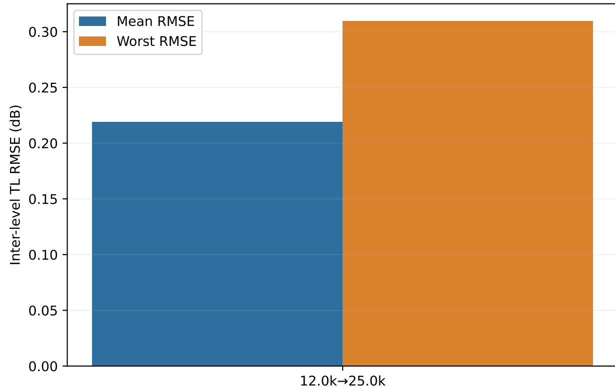
Ray-count convergence
