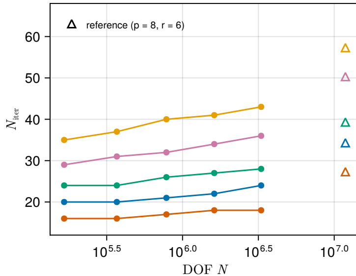
(b) GMRES iterations
