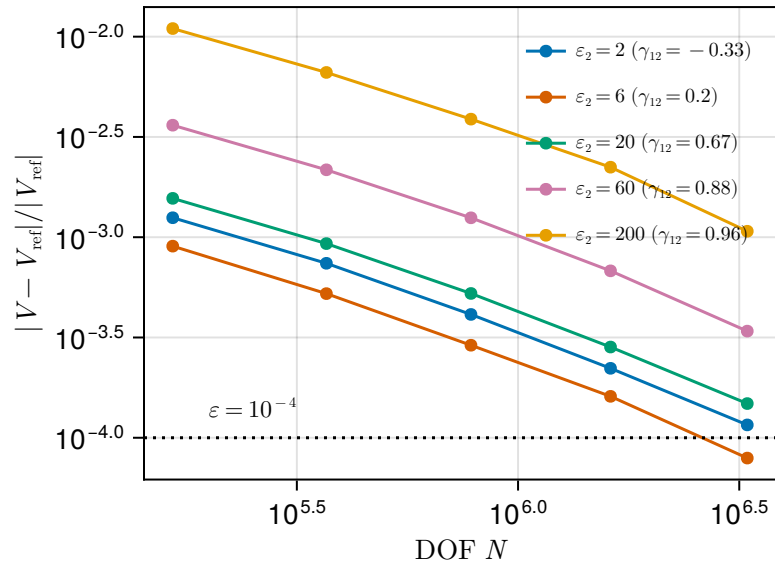
(a) convergence vs contrast ( p = 6 ), \varepsilon = 10^{-4}
