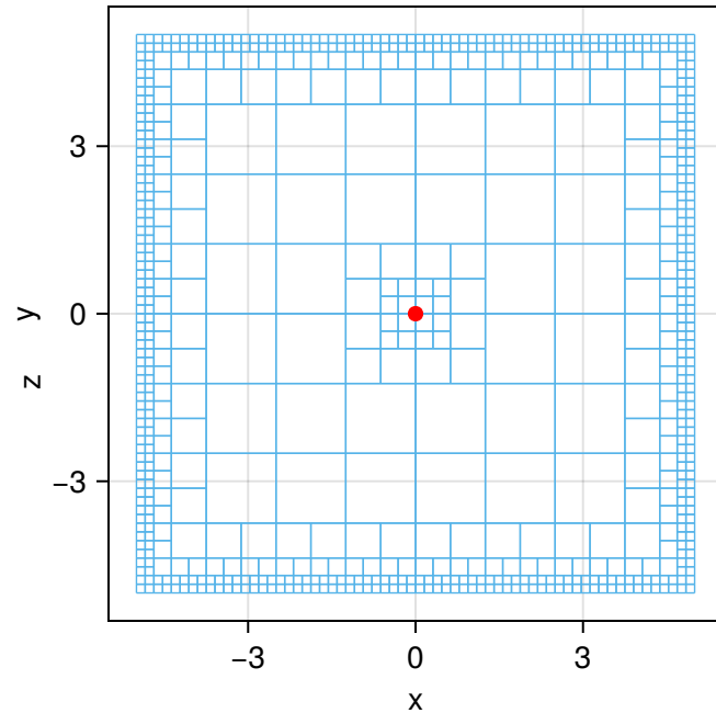
slab top face ( z = 1 ): RHS-adaptive panels
