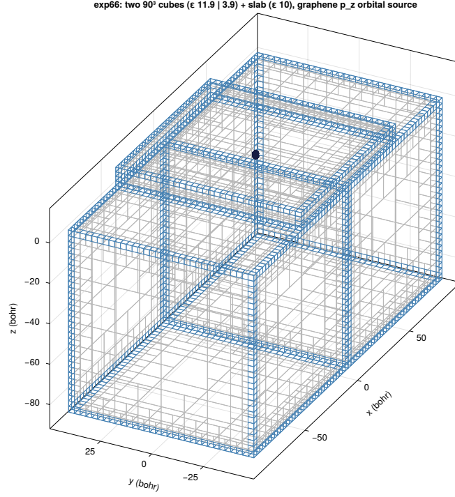
Figure 3: The exp66 multicube system rendered with BL.jl’s Makie extension ( viz_3d ): two 90^3 cubes ( \epsilon = 11.9 | 3.9 ) sharing the buried face, the slab ( \epsilon = 10 ) on top, and the graphene p_z orbital density (dark cluster) at the slab centre over the junction. Coarse interface, visualization only.
