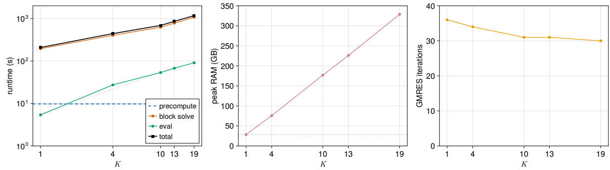
Figure 4: exp66 per-phase runtime (left), peak RAM (centre), and GMRES iteration count (right) versus K . Precompute is K -independent; the block solve is sublinear and the eval linear in K ; peak RAM grows linearly; the block-GMRES iteration count is \sim 30 – 36 (vs. \sim 8 for the single-slab system above).
